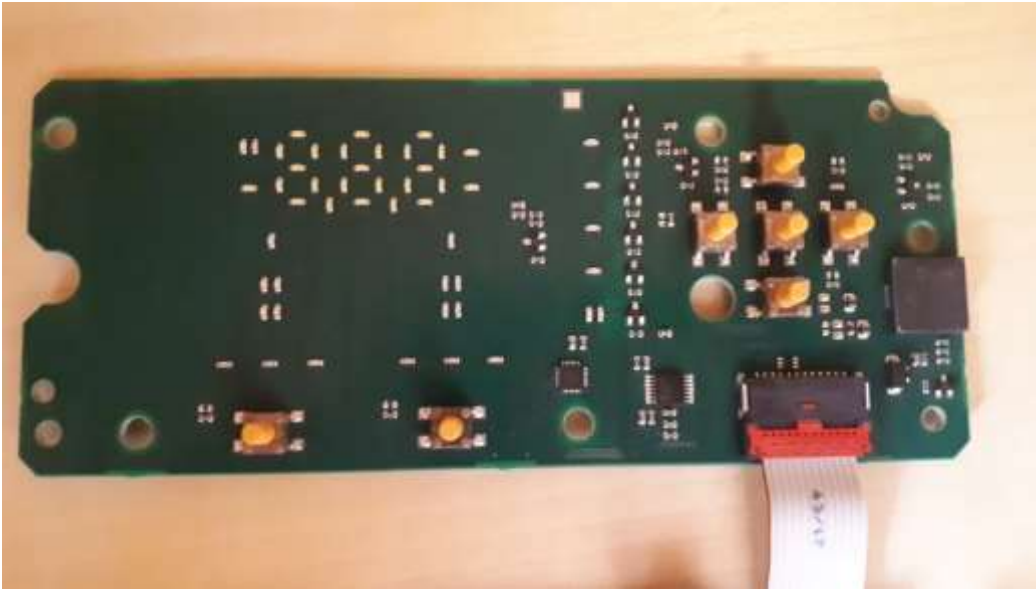
Figure 4 Top view of HMI PCB
