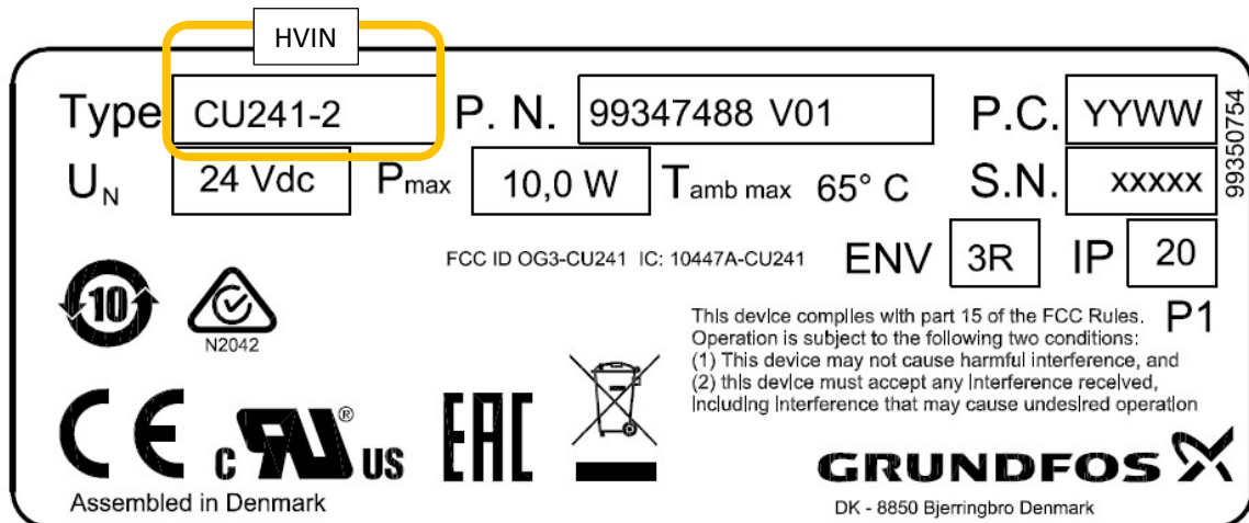
Figure 2 Details of Information on label for CU 241-2
