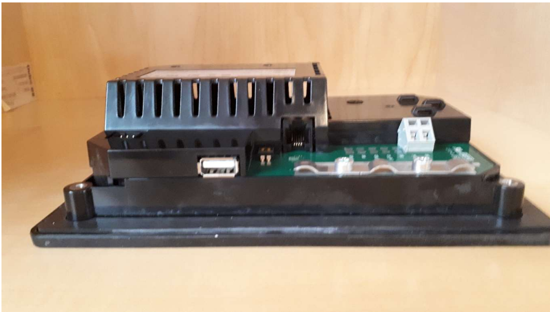
Figure 10 CU 241-X: Bottom view with mounting bracket removed
