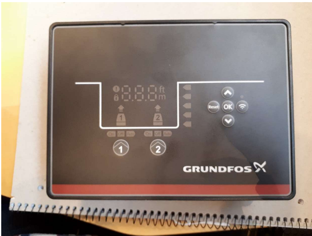
Figure 2 CU 241-2: Front View
