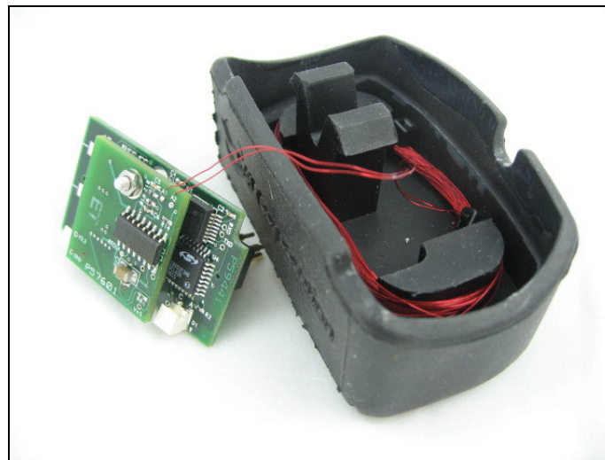
EUT, Partially Disassembled View (Shows Controller and Transceiver PCAs as mated per design.)
