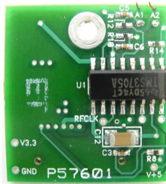
Transceiver PCA Side 2
