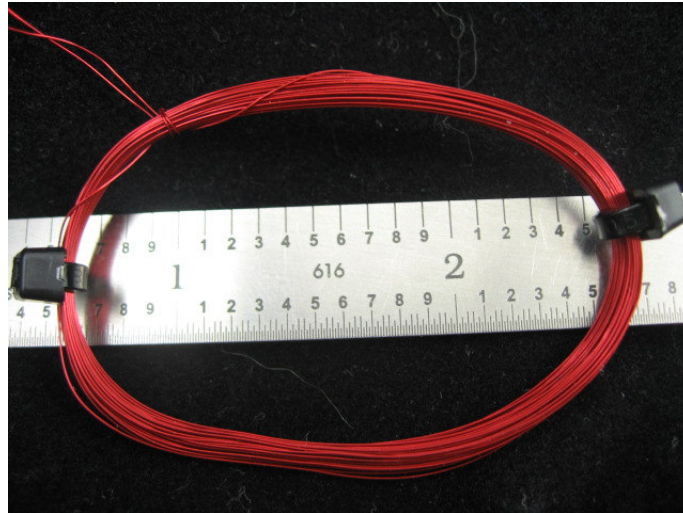
Antenna, Loop
