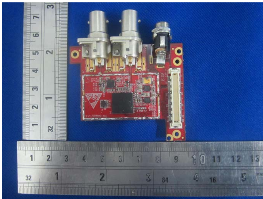
EUT – Sub Board Top Without Copper Foil View
