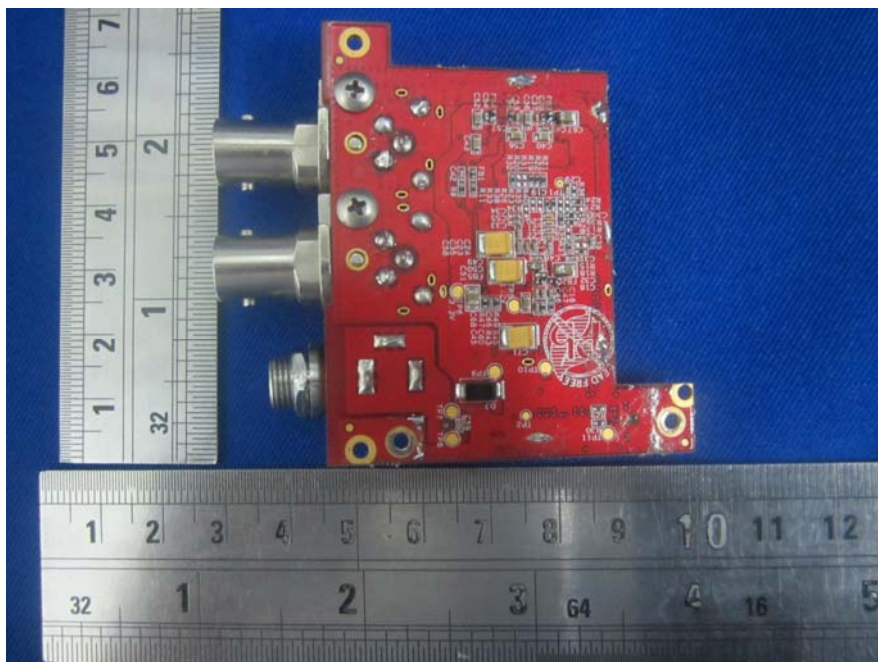
EUT – Sub Board Bottom Without Copper Foil View
