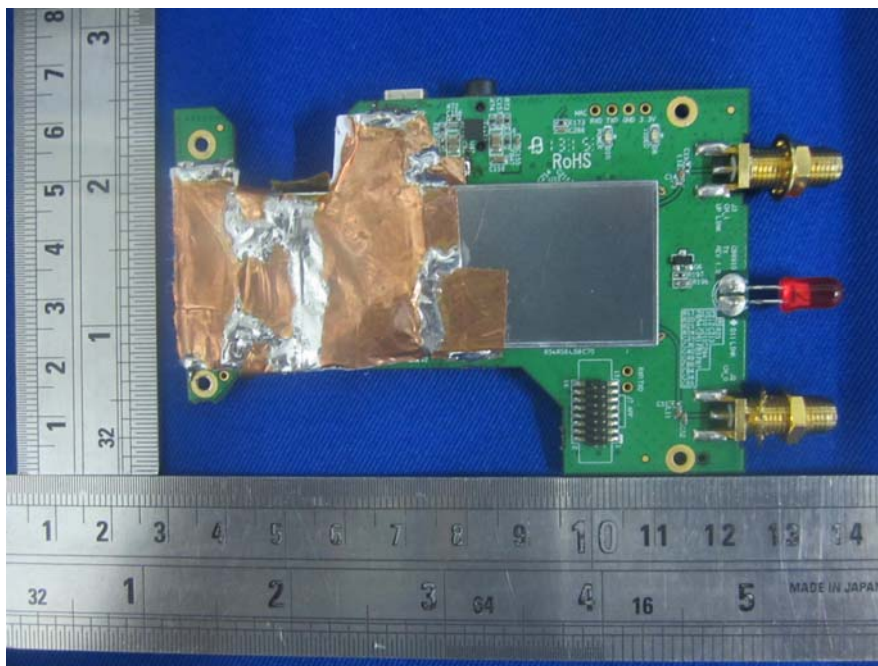
EUT –Main Board Bottom With Copper Foil View
