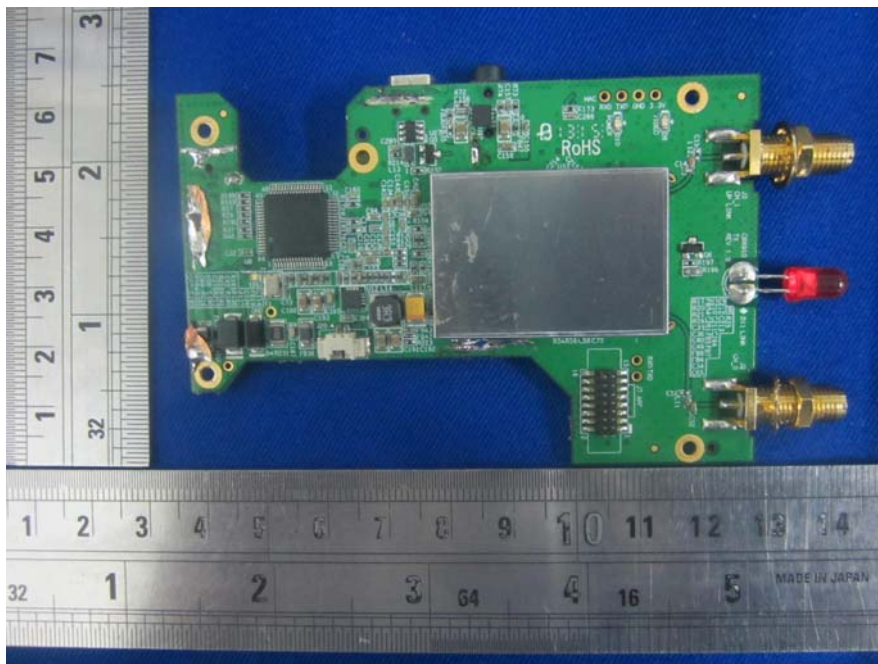
EUT –Main Board Bottom Without Copper Foil View
