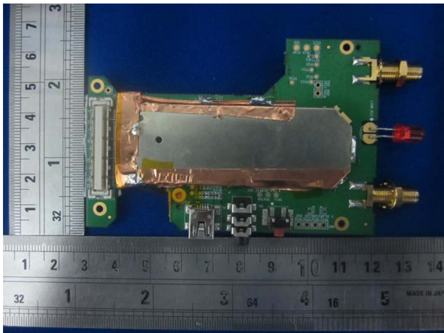
EUT –Main Board Top With Copper Foil View
