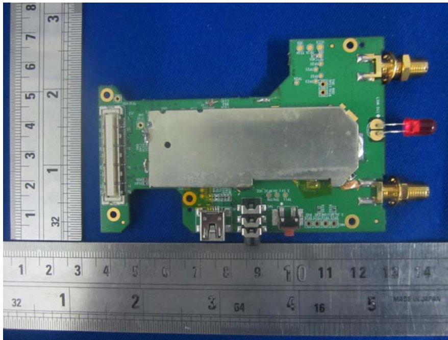
EUT –Main Board Top Without Copper Foil View
