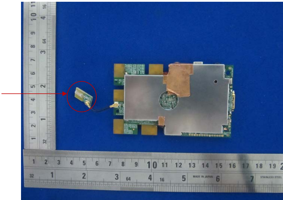
EUT – Main Board Bottom with Shielding View-1
