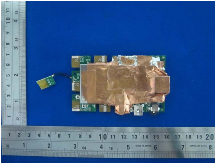
EUT –Main Board Top with Shielding View-1
