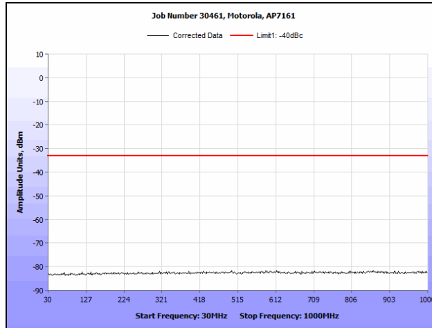
Plot 83. Conducted Spurious Emissions, 802.11a, 4970 MHz (30 MHz - 1 GHz), R3-B
