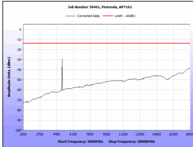
Plot 144. Radiated Spurious Emissions, 802.11n HT20, 4980 MHz (1 GHz – 18 GHz)
