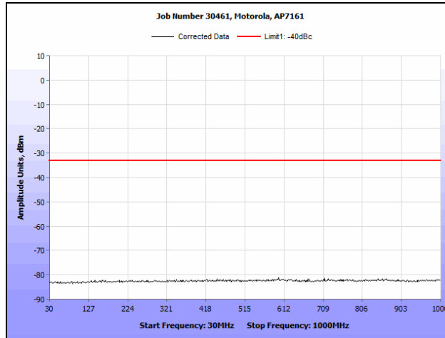
Plot 125. Conducted Spurious Emissions, 802.11n HT20, 4980 MHz (30 MHz – 1 GHz), R3-C
