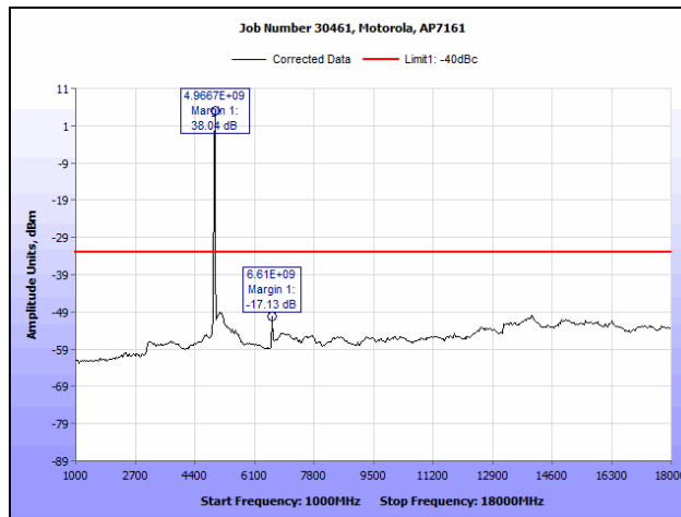
Plot 76. Conducted Spurious Emissions, 802.11a, 4960 MHz (1 GHz – 18 GHz), R3-B
