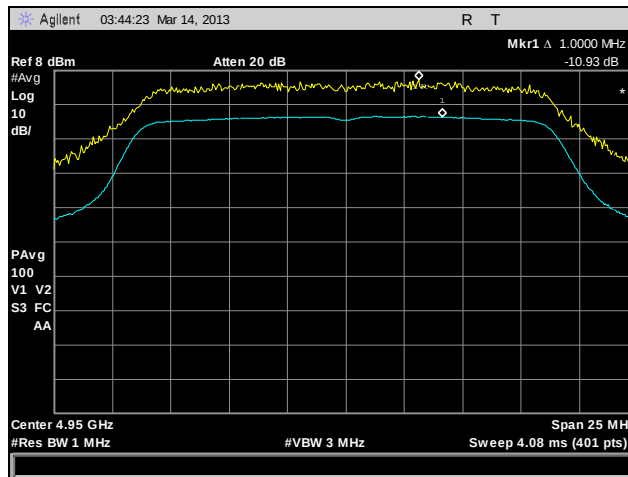
Plot 165. Peak Excursion, 802.11n HT20, 4950 MHz, Port A
