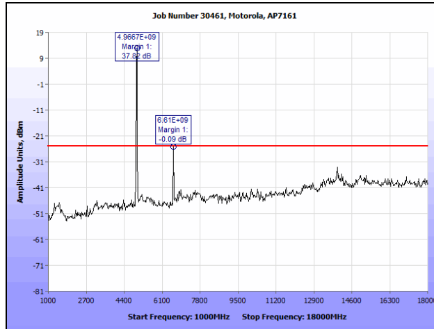
Plot 80. Conducted Spurious Emissions, 802.11a, 4960 MHz (1 GHz – 18 GHz)
