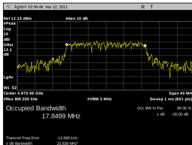
Plot 21. Emission Bandwidth, 802.11n HT20, 4970 MHz, Port C (3x3)
