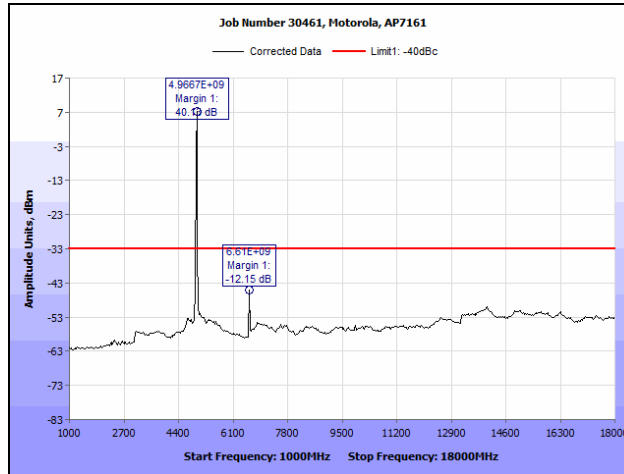
Plot 74. Conducted Spurious Emissions, 802.11a, 4960 MHz (1 GHz – 18 GHz), R3-A
