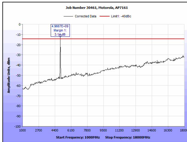
Plot 147. Radiated Spurious Emissions, 802.11a, 4970 MHz (1 GHz – 18 GHz), (1x1)
