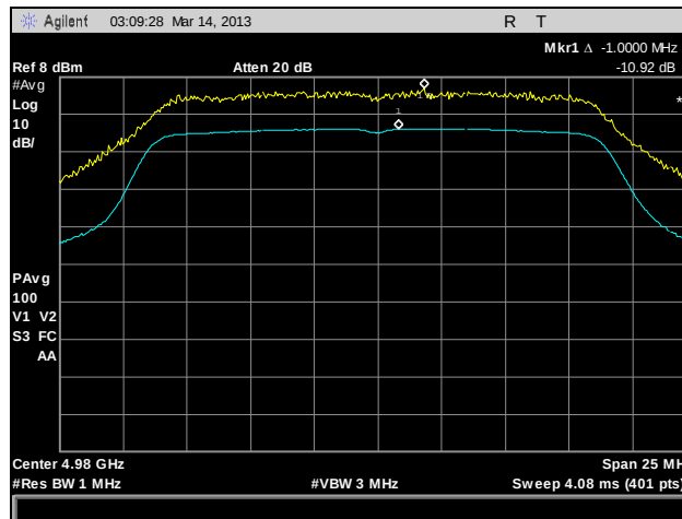
Plot 174. Peak Excursion, 802.11n HT20, 4980 MHz, Port A
