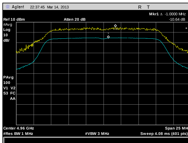
Plot 178. Peak Excursion, 802.11a, 4960 MHz, 1x1
