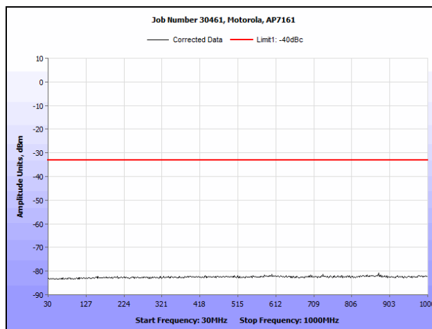
Plot 109. Conducted Spurious Emissions, 802.11n HT20, 4960 MHz (30 MHz - 1 GHz), R3-C
