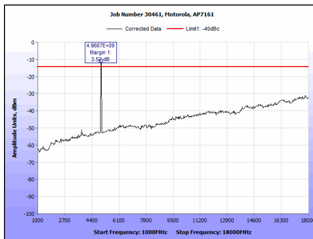
Plot 148. Radiated Spurious Emissions, 802.11a, 4980 MHz (1 GHz – 18 GHz), (1x1)
