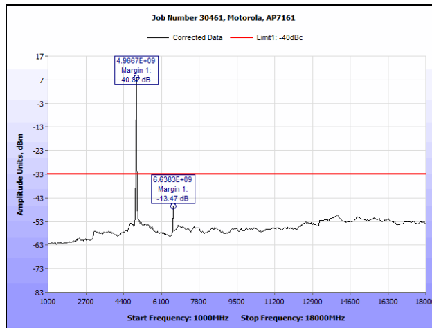
Plot 82. Conducted Spurious Emissions, 802.11a, 4970 MHz (1 GHz – 18 GHz), R3-A
