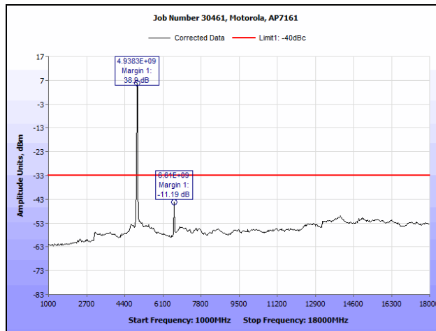
Plot 98. Conducted Spurious Emissions, 802.11n HT20, 4950 MHz (1 GHz – 18 GHz), R3-A
