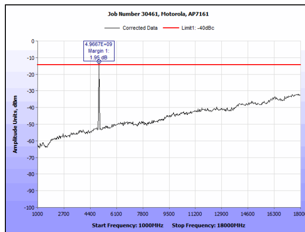
Plot 151. Radiated Spurious Emissions, 802.11n HT20, 4970 MHz (1 GHz – 18 GHz), (1x1)
