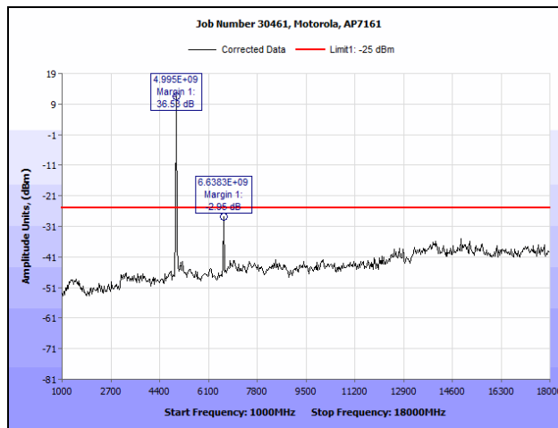
Plot 96. Conducted Spurious Emissions, 802.11a, 4980 MHz (1 GHz – 18 GHz)
