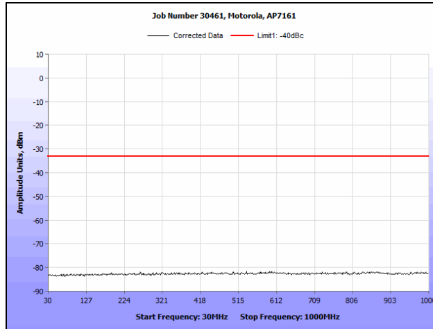
Plot 101. Conducted Spurious Emissions, 802.11n HT20, 4950 MHz (30 MHz – 1 GHz), R3-C
