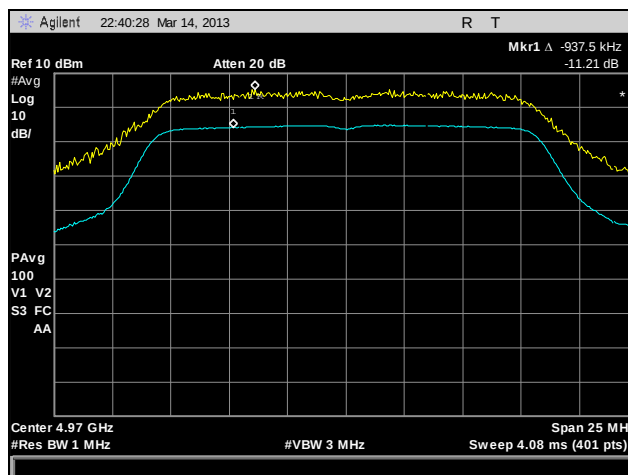
Plot 179. Peak Excursion, 802.11a, 4970 MHz, 1x1
