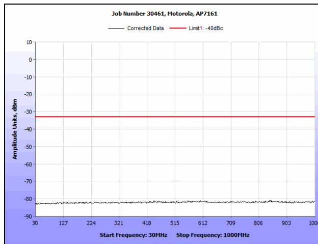
Plot 81. Conducted Spurious Emissions, 802.11a, 4970 MHz (30 MHz – 1 GHz), R3-A
