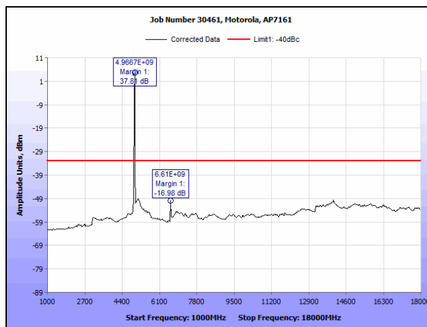
Plot 108. Conducted Spurious Emissions, 802.11n HT20, 4960 MHz (1 GHz - 18 GHz), R3-B
