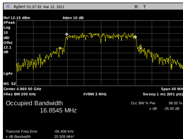
Plot 5. Emission Bandwidth, 802.11a, 4960 MHz, Port B (3x3)
