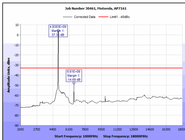
Plot 70. Conducted Spurious Emissions, 802.11a, 4950 MHz (1 GHz – 18 GHz), R3-C
