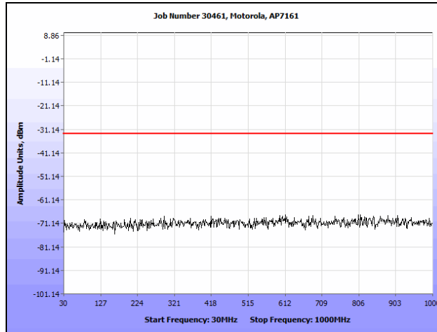
Plot 119. Conducted Spurious Emissions, 802.11n HT20, 4970 MHz (30 MHz – 1 GHz)
