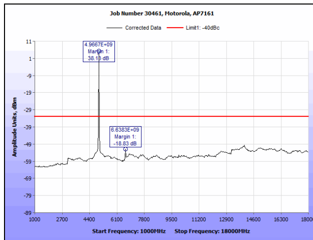
Plot 126. Conducted Spurious Emissions, 802.11n HT20, 4980 MHz (1 GHz – 18 GHz), R3-C
