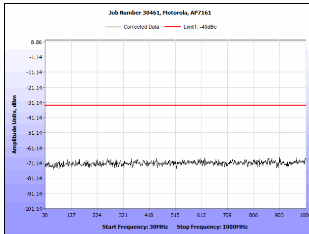
Plot 127. Conducted Spurious Emissions, 802.11n HT20, 4980 MHz (30 MHz – 1 GHz)
