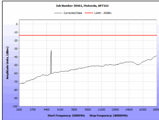
Plot 132. Radiated Spurious Emissions, 802.11a, 4960 MHz (1 GHz – 18 GHz)
