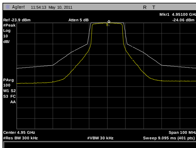
Plot 34. Emission Mask, 802.11a, 4950 MHz, Port B (3x3)
