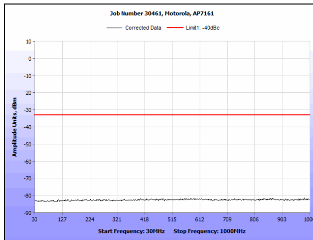
Plot 117. Conducted Spurious Emissions, 802.11n HT20, 4970 MHz (30 MHz – 1 GHz), R3-C
