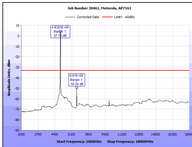
Plot 102. Conducted Spurious Emissions, 802.11n HT20, 4950 MHz (1 GHz – 18 GHz), R3-C
