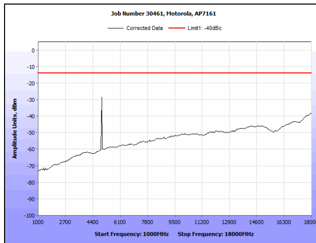
Plot 136. Radiated Spurious Emissions, 802.11a, 4980 MHz (1 GHz – 18 GHz)
