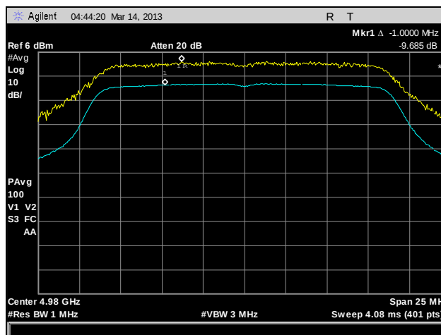
Plot 175. Peak Excursion, 802.11n HT20, 4980 MHz, Port B
