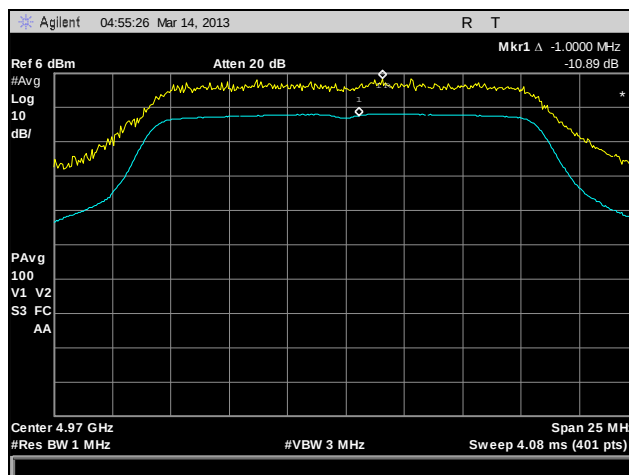
Plot 161. Peak Excursion, 802.11a, 4970 MHz, Port C
