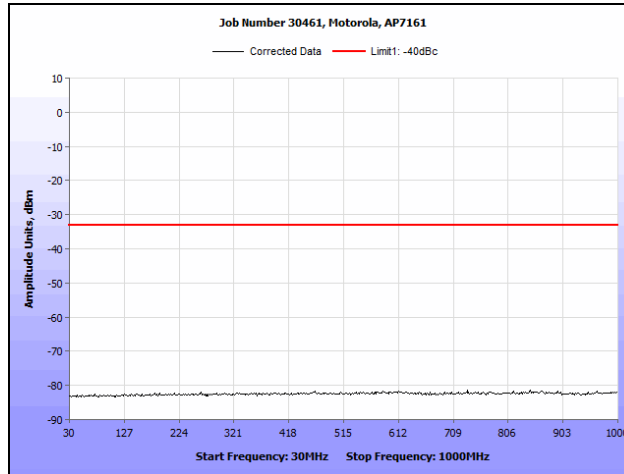
Plot 77. Conducted Spurious Emissions, 802.11a, 4960 MHz (30 MHz – 1 GHz), R3-C
