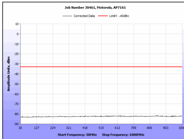
Plot 85. Conducted Spurious Emissions, 802.11a, 4970 MHz (30 MHz - 1 GHz), R3-C
