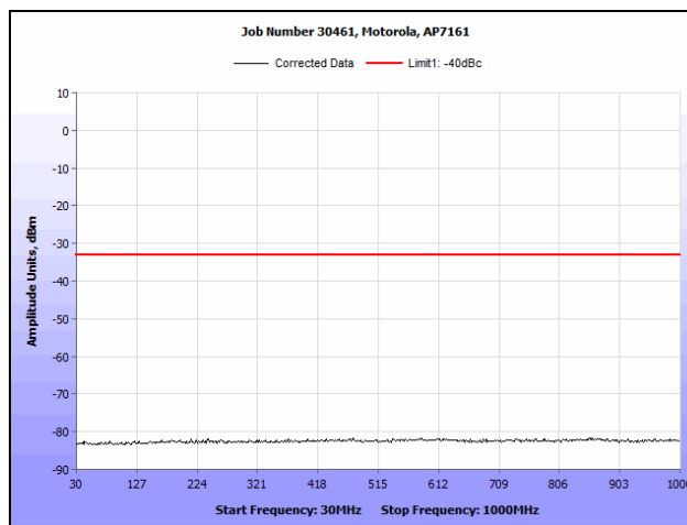
Plot 99. Conducted Spurious Emissions, 802.11n HT20, 4950 MHz (30 MHz - 1 GHz), R3-B
