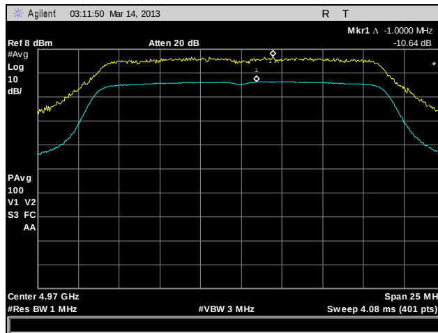
Plot 171. Peak Excursion, 802.11n HT20, 4970 MHz, Port A
