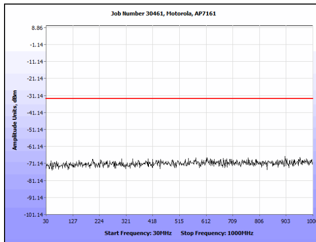
Plot 87. Conducted Spurious Emissions, 802.11a, 4970 MHz (30 MHz – 1 GHz)
