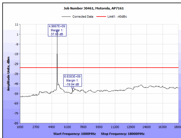
Plot 124. Conducted Spurious Emissions, 802.11n HT20, 4980 MHz (1 GHz – 18 GHz), R3-B
