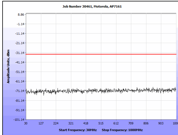
Plot 71. Conducted Spurious Emissions, 802.11a, 4950 MHz (30 MHz – 1 GHz)
