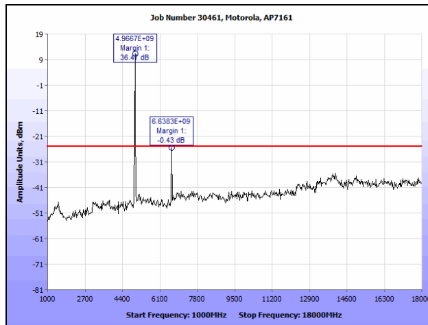
Plot 88. Conducted Spurious Emissions, 802.11a, 4970 MHz (1 GHz – 18 GHz)
