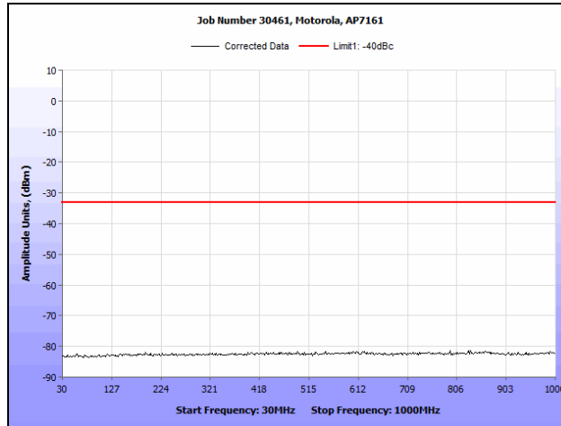
Plot 113. Conducted Spurious Emissions, 802.11n HT20, 4970 MHz (30 MHz – 1 GHz), R3-A
