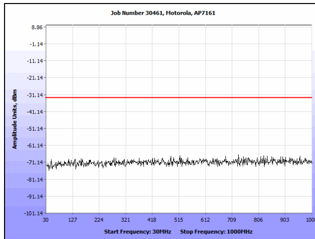
Plot 103. Conducted Spurious Emissions, 802.11n HT20, 4950 MHz (30 MHz – 1 GHz)
