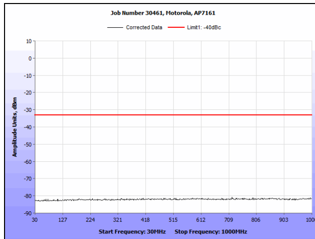
Plot 73. Conducted Spurious Emissions, 802.11a, 4960 MHz (30 MHz – 1 GHz), R3-A
