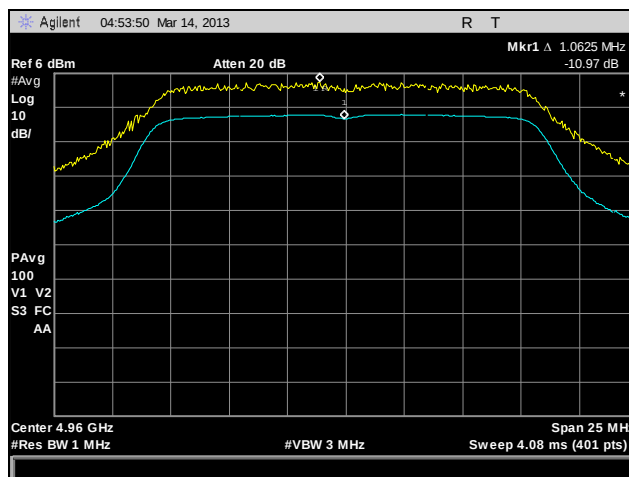
Plot 158. Peak Excursion, 802.11a, 4960 MHz, Port C
