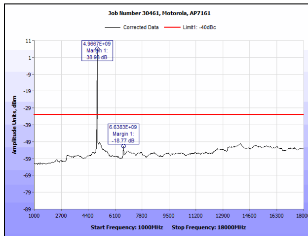
Plot 84. Conducted Spurious Emissions, 802.11a, 4970 MHz (1 GHz - 18 GHz), R3-B
