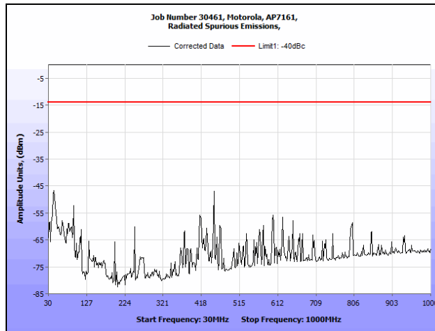
Plot 129. Radiated Spurious Emissions, 802.11a, 4950 MHz (30 MHz – 1 GHz)
