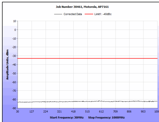
Plot 75. Conducted Spurious Emissions, 802.11a, 4960 MHz (30 MHz - 1 GHz), R3-B
