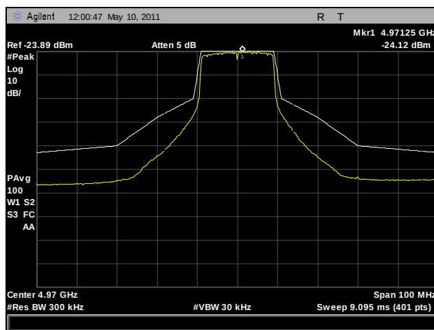
Plot 52. Emission Mask, 802.11n HT20, 4970 MHz, Port B (3x3)
