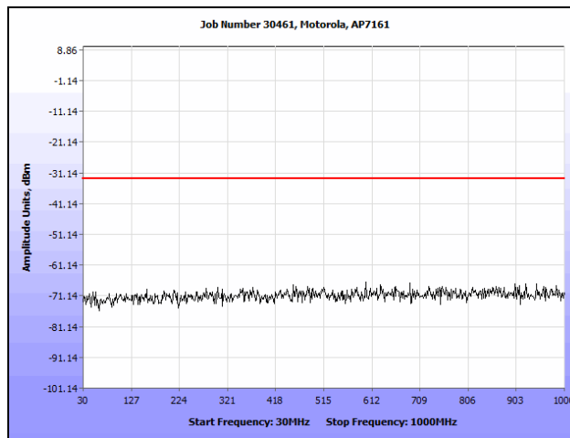
Plot 111. Conducted Spurious Emissions, 802.11n HT20, 4960 MHz (30 MHz – 1 GHz)
