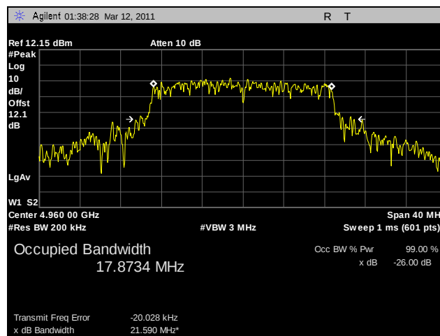
Plot 17. Emission Bandwidth, 802.11n HT20, 4960 MHz, Port B (3x3)
