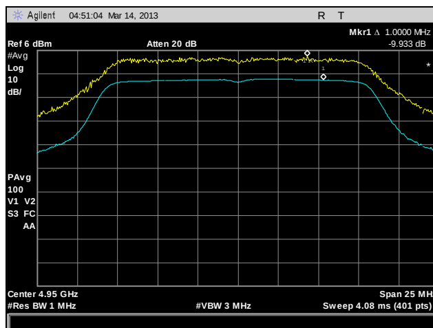
Plot 155. Peak Excursion, 802.11a, 4950 MHz, Port C
