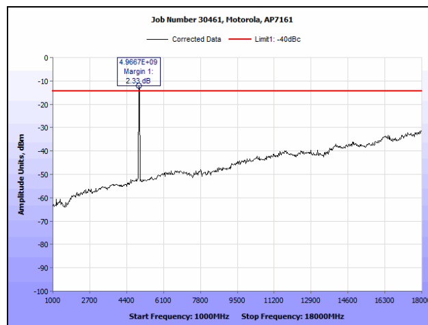
Plot 152. Radiated Spurious Emissions, 802.11n HT20, 4980 MHz (1 GHz – 18 GHz), (1x1)
