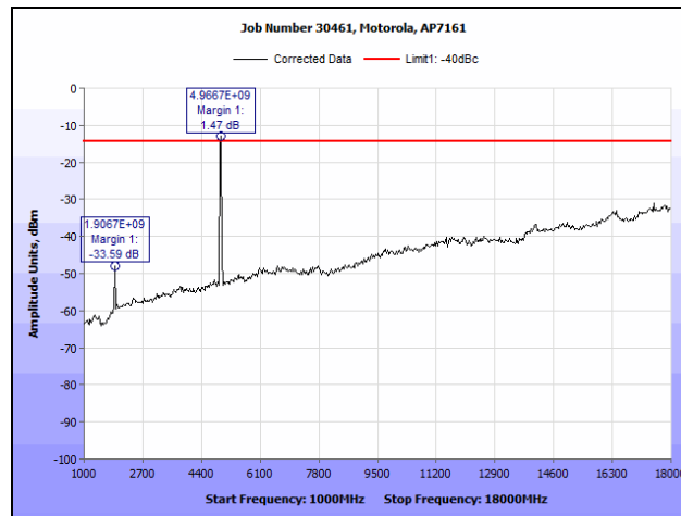
Plot 150. Radiated Spurious Emissions, 802.11n HT20, 4960 MHz (1 GHz – 18 GHz), (1x1)
