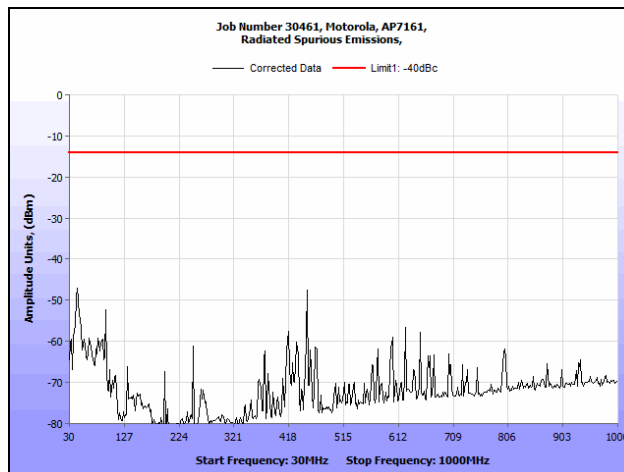
Plot 131. Radiated Spurious Emissions, 802.11a, 4960 MHz (30 MHz – 1 GHz)
