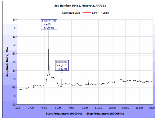
Plot 110. Conducted Spurious Emissions, 802.11n HT20, 4960 MHz (1 GHz – 18 GHz), R3-C
