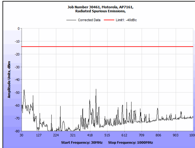
Plot 141. Radiated Spurious Emissions, 802.11n HT20, 4970 MHz (30 MHz – 1 GHz)
