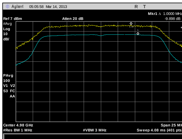
Plot 176. Peak Excursion, 802.11n HT20, 4980 MHz, Port C
