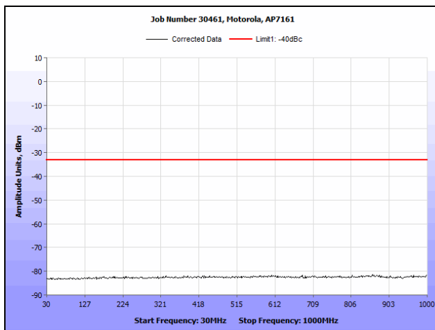
Plot 89. Conducted Spurious Emissions, 802.11a, 4980 MHz (30 MHz – 1 GHz), R3-A
