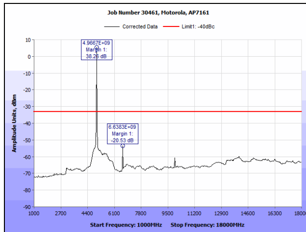
Plot 94. Conducted Spurious Emissions, 802.11a, 4980 MHz (1 GHz – 18 GHz), R3-C
