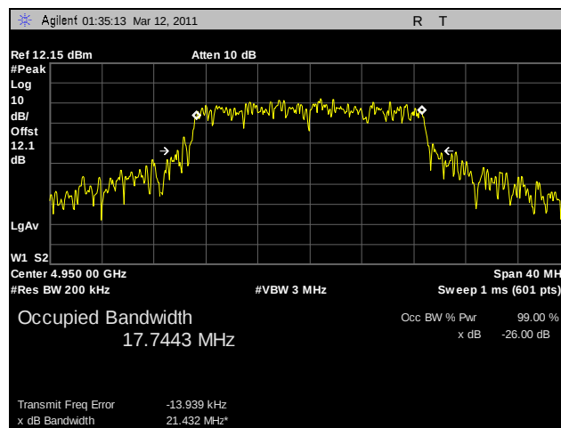
Plot 14. Emission Bandwidth, 802.11n HT20, 4950 MHz, Port B (3x3)
