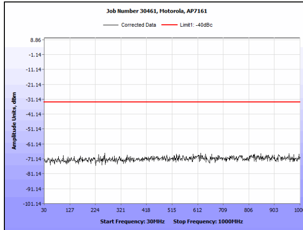
Plot 95. Conducted Spurious Emissions, 802.11a, 4980 MHz (30 MHz – 1 GHz)
