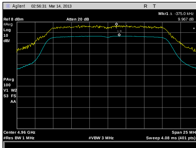
Plot 156. Peak Excursion, 802.11a, 4960 MHz, Port A
