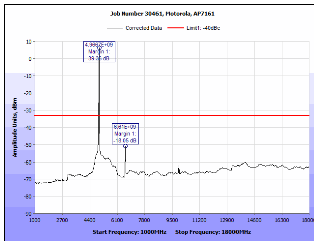
Plot 78. Conducted Spurious Emissions, 802.11a, 4960 MHz (1 GHz – 18 GHz), R3-C
