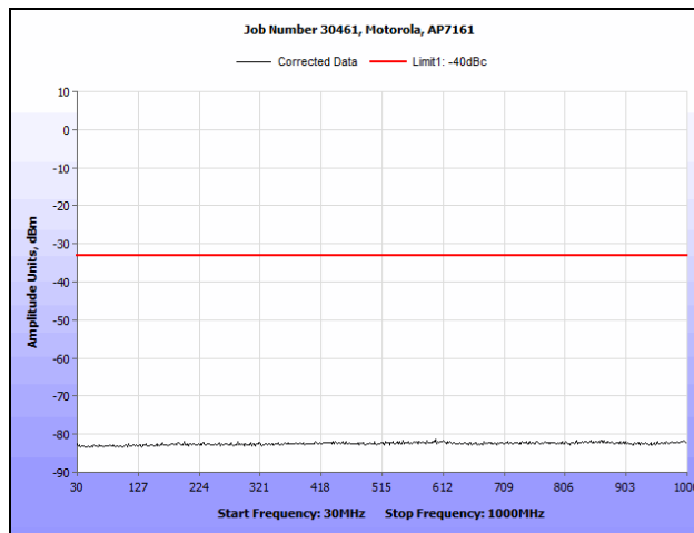
Plot 93. Conducted Spurious Emissions, 802.11a, 4980 MHz (30 MHz – 1 GHz), R3-C
