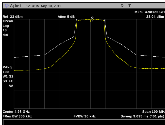
Plot 55. Emission Mask, 802.11n HT20, 4980 MHz, Port B (3x3)
