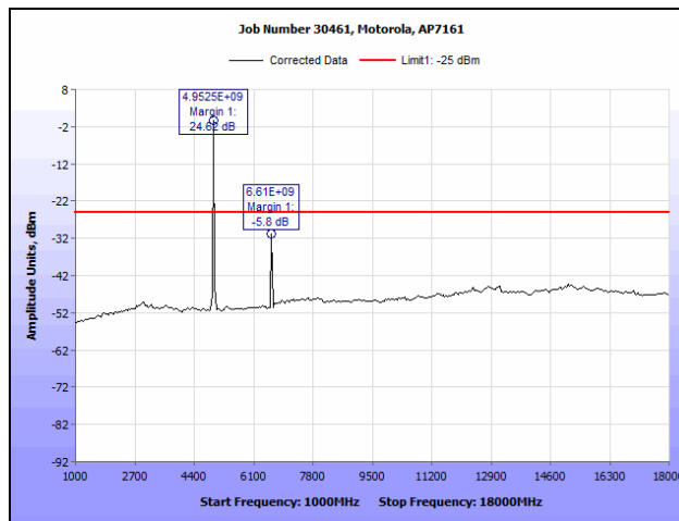
Plot 72. Conducted Spurious Emissions, 802.11a, 4950 MHz (1 GHz – 18 GHz)
