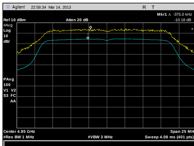
Plot 181. Peak Excursion, 802.11n HT20, 4950 MHz, 1x1
