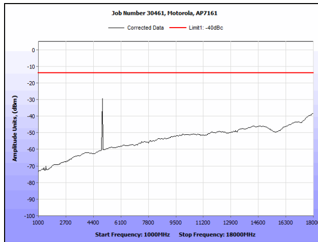
Plot 134. Radiated Spurious Emissions, 802.11a, 4970 MHz (1 GHz – 18 GHz)
