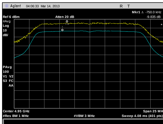
Plot 166. Peak Excursion, 802.11n HT20, 4950 MHz, Port B
