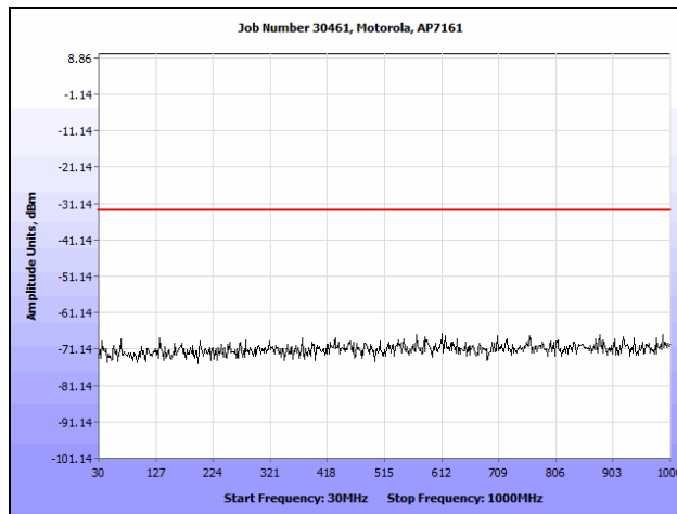
Plot 79. Conducted Spurious Emissions, 802.11a, 4960 MHz (30 MHz – 1 GHz)
