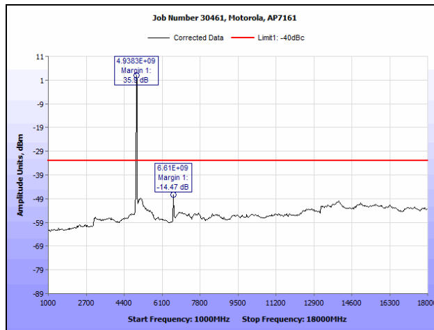
Plot 68. Conducted Spurious Emissions, 802.11a, 4950 MHz (1 GHz – 18 GHz), R3-B
