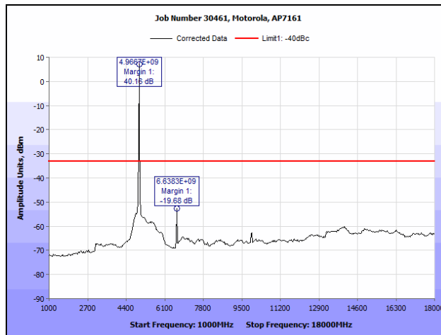
Plot 118. Conducted Spurious Emissions, 802.11n HT20, 4970 MHz (1 GHz – 18 GHz), R3-C
