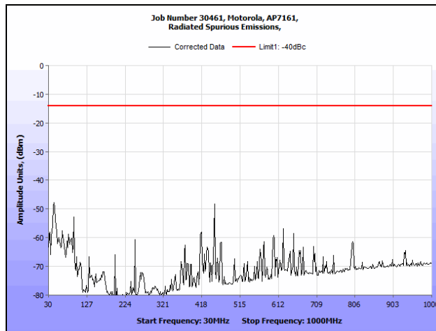
Plot 143. Radiated Spurious Emissions, 802.11n HT20, 4980 MHz (30 MHz – 1 GHz)
