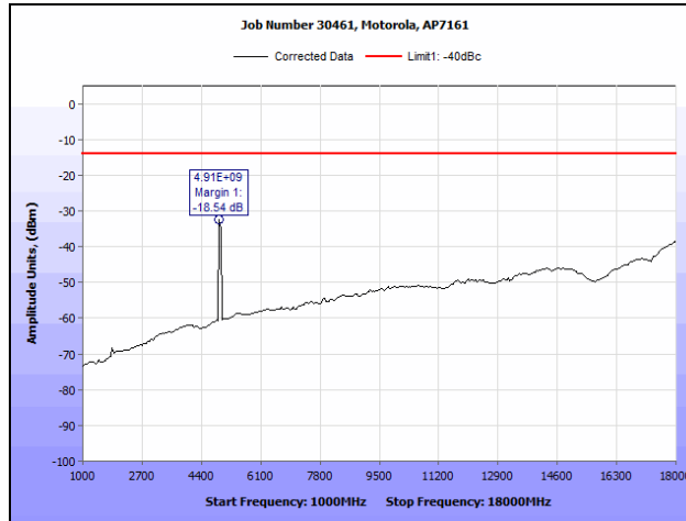
Plot 138. Radiated Spurious Emissions, 802.11n HT20, 4950 MHz (1 GHz – 18 GHz)
