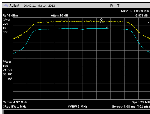
Plot 172. Peak Excursion, 802.11n HT20, 4970 MHz, Port B
