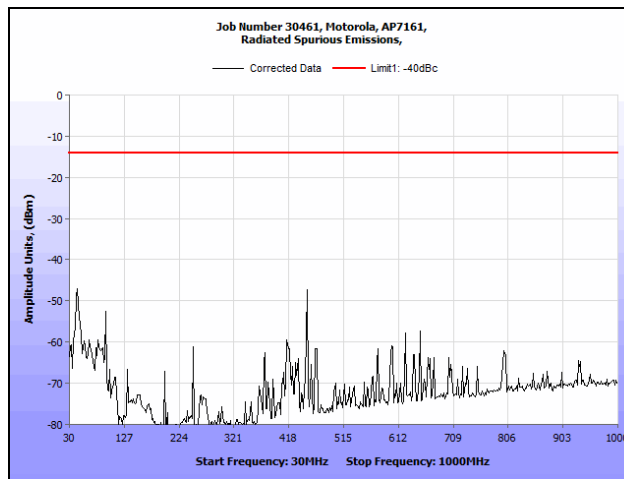
Plot 133. Radiated Spurious Emissions, 802.11a, 4970 MHz (30 MHz – 1 GHz)
