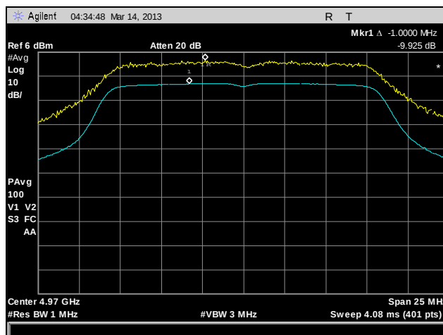
Plot 160. Peak Excursion, 802.11a, 4970 MHz, Port B
