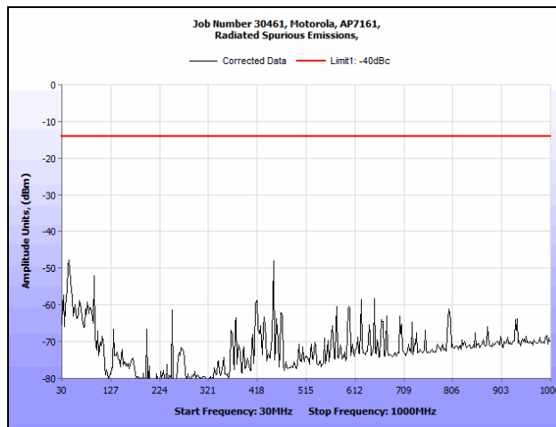
Plot 139. Radiated Spurious Emissions, 802.11n HT20, 4960 MHz (30 MHz – 1 GHz)
