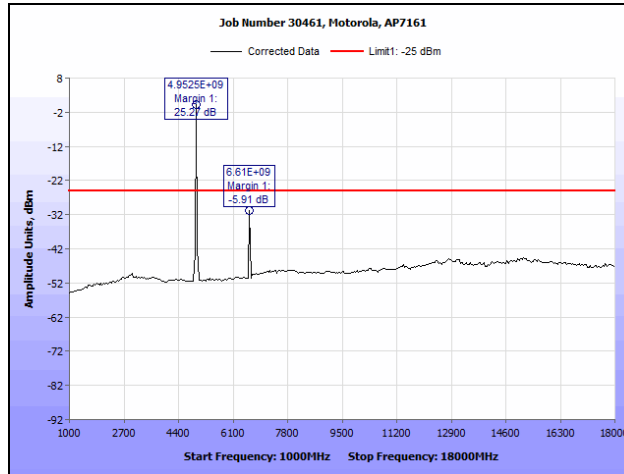
Plot 104. Conducted Spurious Emissions, 802.11n HT20, 4950 MHz (1 GHz – 18 GHz)
