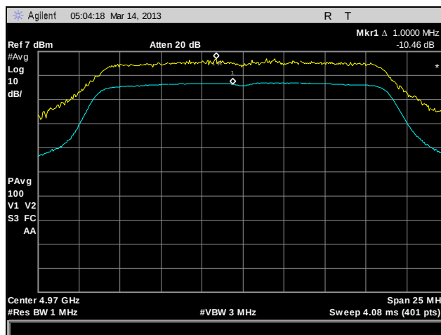
Plot 173. Peak Excursion, 802.11n HT20, 4970 MHz, Port C
