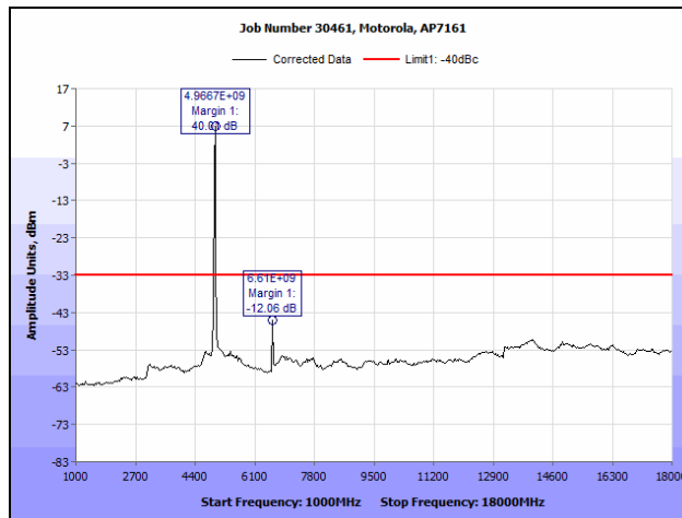
Plot 106. Conducted Spurious Emissions, 802.11n HT20, 4960 MHz (1 GHz – 18 GHz), R3-A
