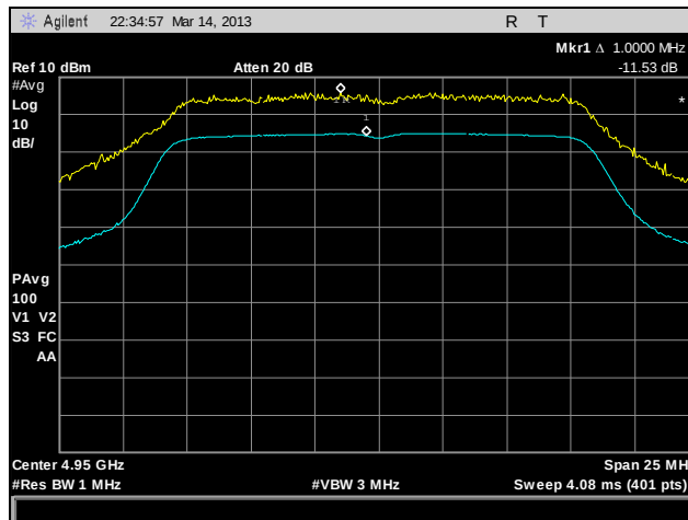
Plot 177. Peak Excursion, 802.11a, 4950 MHz, 1x1
