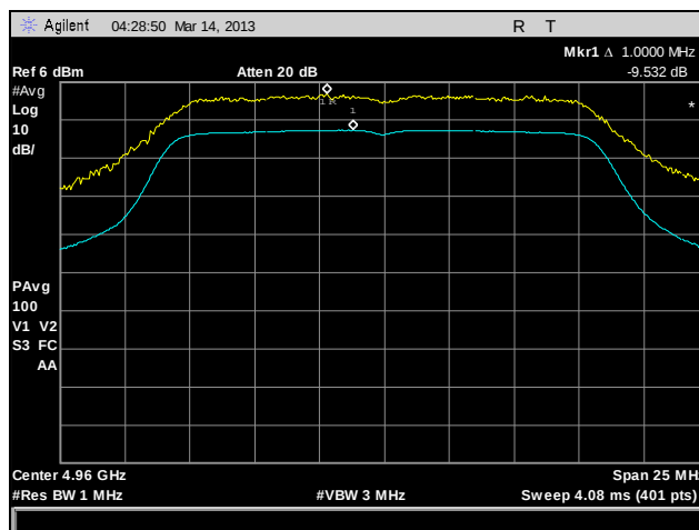
Plot 157. Peak Excursion, 802.11a, 4960 MHz, Port B
