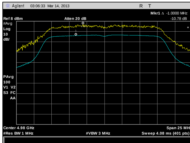
Plot 162. Peak Excursion, 802.11a, 4980 MHz, Port A
