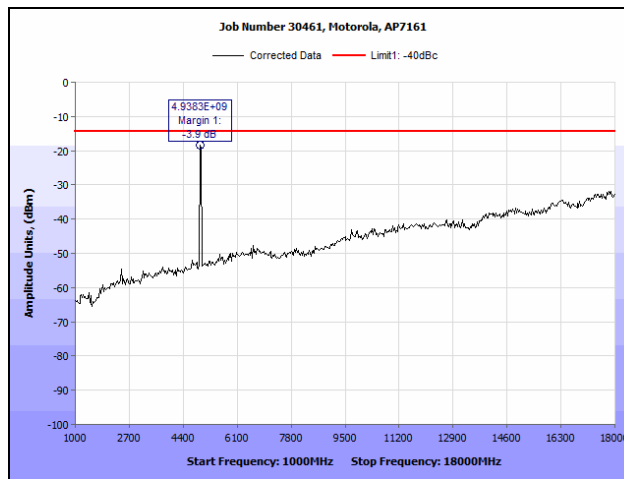
Plot 145. Radiated Spurious Emissions, 802.11a, 4950 MHz (1 GHz – 18 GHz), (1x1)
