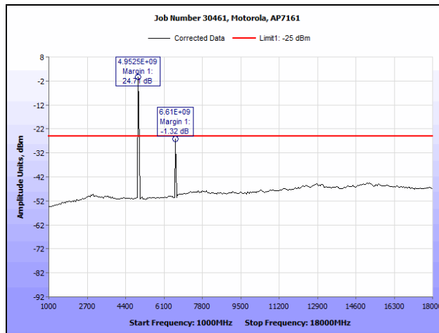
Plot 112. Conducted Spurious Emissions, 802.11n HT20, 4960 MHz (1 GHz – 18 GHz)
