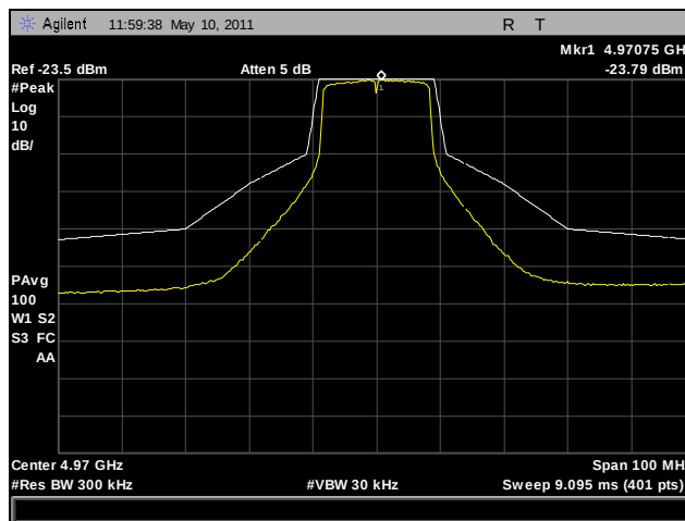
Plot 40. Emission Mask, 802.11a, 4970 MHz, Port B (3x3)
