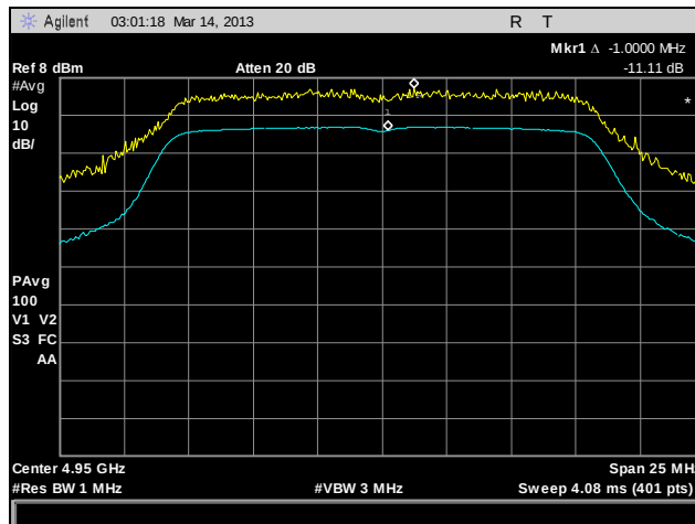
Plot 153. Peak Excursion, 802.11a, 4950 MHz, Port A
