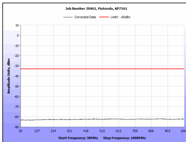
Plot 69. Conducted Spurious Emissions, 802.11a, 4950 MHz (30 MHz – 1 GHz), R3-C
