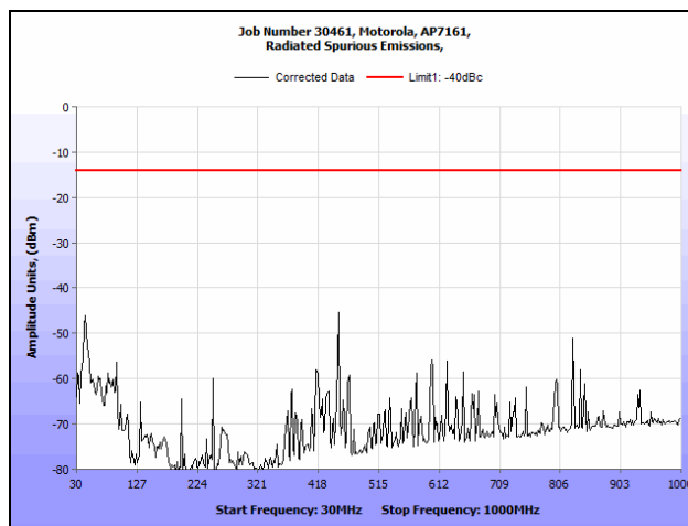
Plot 137. Radiated Spurious Emissions, 802.11n HT20, 4950 MHz (30 MHz – 1 GHz)
