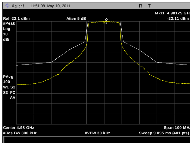
Plot 54. Emission Mask, 802.11n HT20, 4980 MHz, Port A (3x3)
