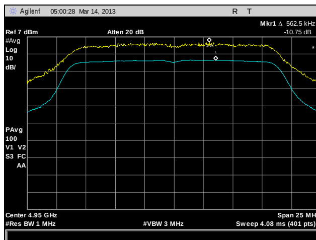
Plot 167. Peak Excursion, 802.11n HT20, 4950 MHz, Port C
