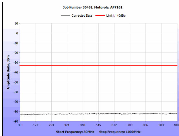
Plot 67. Conducted Spurious Emissions, 802.11a, 4950 MHz (30 MHz - 1 GHz), R3-B
