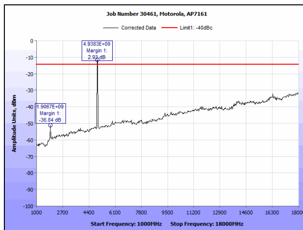
Plot 149. Radiated Spurious Emissions, 802.11n HT20, 4950 MHz (1 GHz – 18 GHz), (1x1)
