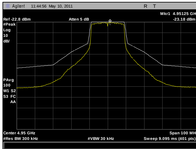
Plot 45. Emission Mask, 802.11n HT20, 4950 MHz, Port A (3x3)
