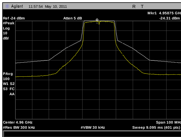
Plot 49. Emission Mask, 802.11n HT20, 4960 MHz, Port B (3x3)
