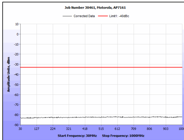
Plot 121. Conducted Spurious Emissions, 802.11n HT20, 4980 MHz (30 MHz – 1 GHz), R3-A
