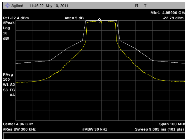
Plot 36. Emission Mask, 802.11a, 4960 MHz, Port A (3x3)
