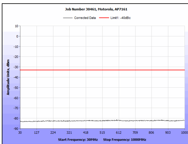
Plot 91. Conducted Spurious Emissions, 802.11a, 4980 MHz (30 MHz – 1 GHz), R3-B
