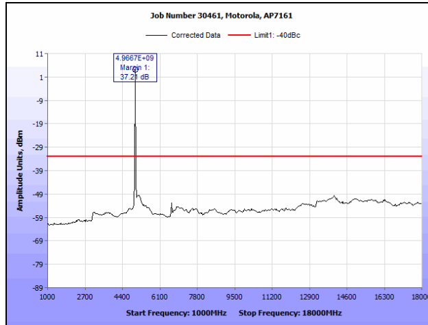
Plot 92. Conducted Spurious Emissions, 802.11a, 4980 MHz (1 GHz – 18 GHz), R3-B
