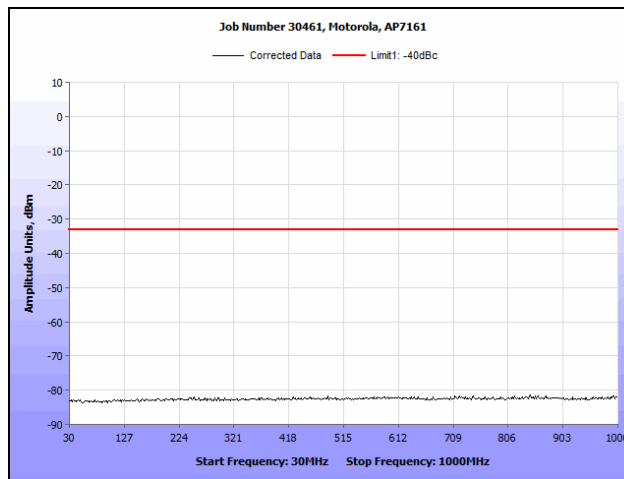
Plot 105. Conducted Spurious Emissions, 802.11n HT20, 4960 MHz (30 MHz – 1 GHz), R3-A
