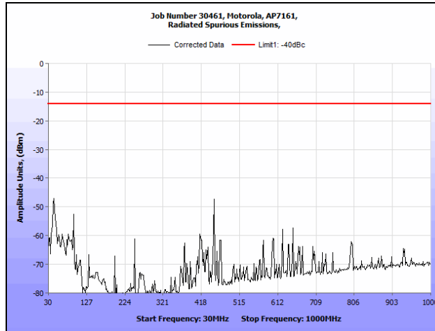
Plot 135. Radiated Spurious Emissions, 802.11a, 4980 MHz (30 MHz – 1 GHz)
