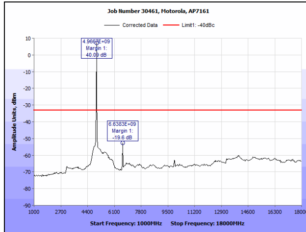
Plot 86. Conducted Spurious Emissions, 802.11a, 4970 MHz (1 GHz – 18 GHz), R3-C
