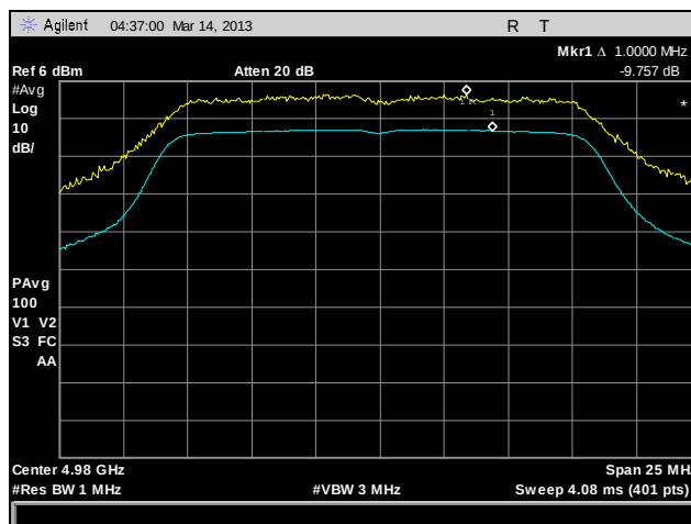
Plot 163. Peak Excursion, 802.11a, 4980 MHz, Port B
