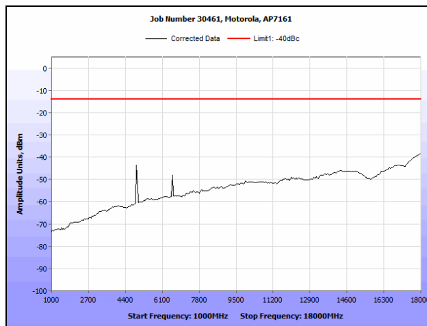
Plot 130. Radiated Spurious Emissions, 802.11a, 4950 MHz (1 GHz – 18 GHz)
