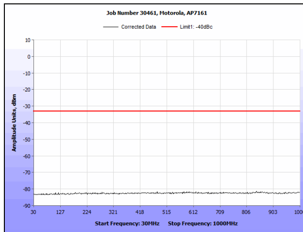
Plot 123. Conducted Spurious Emissions, 802.11n HT20, 4980 MHz (30 MHz - 1 GHz), R3-B
