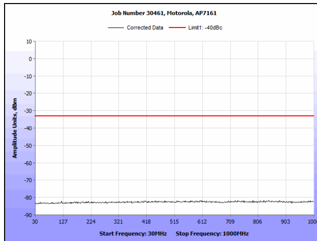
Plot 97. Conducted Spurious Emissions, 802.11n HT20, 4950 MHz (30 MHz – 1 GHz), R3-A
