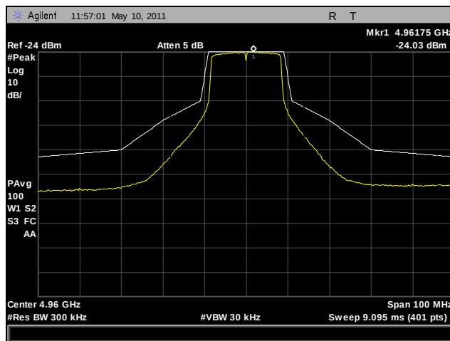
Plot 37. Emission Mask, 802.11a, 4960 MHz, Port B (3x3)
