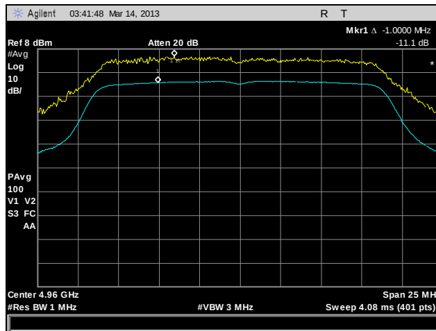
Plot 168. Peak Excursion, 802.11n HT20, 4960 MHz, Port A
