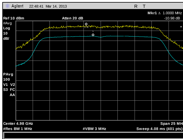
Plot 184. Peak Excursion, 802.11n HT20, 4980 MHz, 1x1
