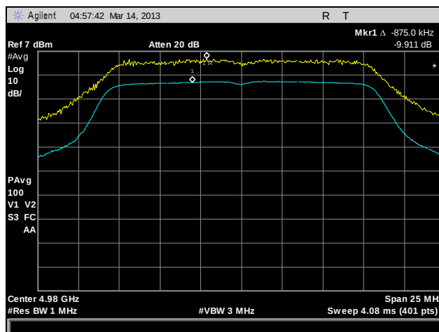
Plot 164. Peak Excursion, 802.11a, 4980 MHz, Port C
