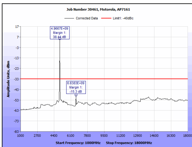
Plot 90. Conducted Spurious Emissions, 802.11a, 4980 MHz (1 GHz – 18 GHz), R3-A
