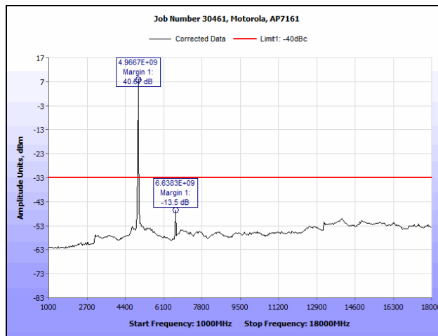
Plot 114. Conducted Spurious Emissions, 802.11n HT20, 4970 MHz (1 GHz – 18 GHz), R3-A
