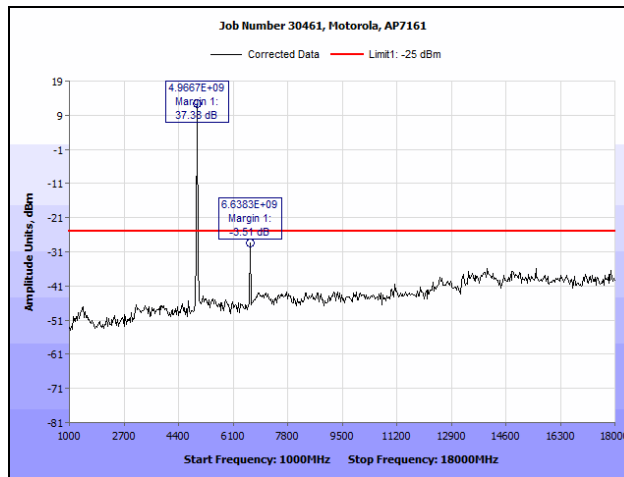
Plot 128. Conducted Spurious Emissions, 802.11n HT20, 4980 MHz (1 GHz – 18 GHz)
