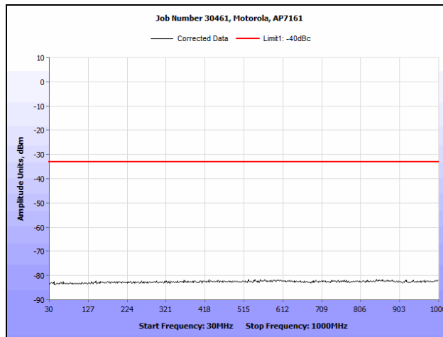
Plot 107. Conducted Spurious Emissions, 802.11n HT20, 4960 MHz (30 MHz - 1 GHz), R3-B
