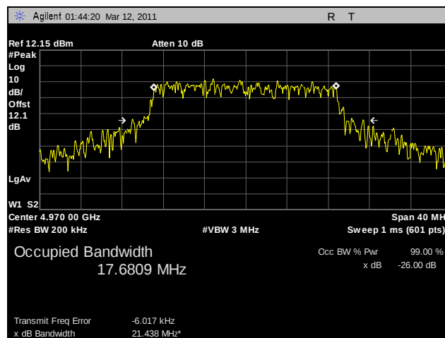
Plot 20. Emission Bandwidth, 802.11n HT20, 4970 MHz, Port B (3x3)
