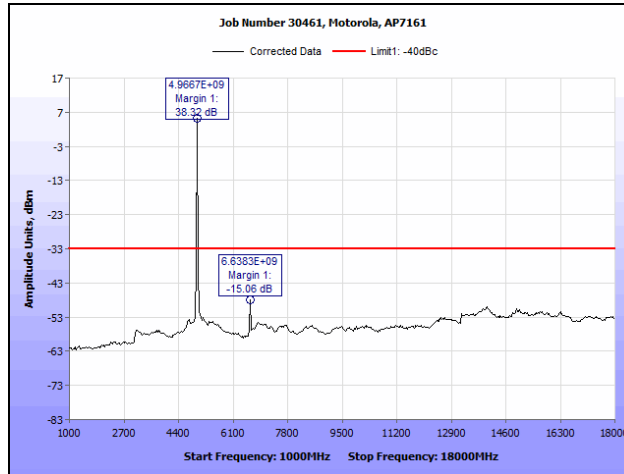
Plot 122. Conducted Spurious Emissions, 802.11n HT20, 4980 MHz (1 GHz – 18 GHz), R3-A
