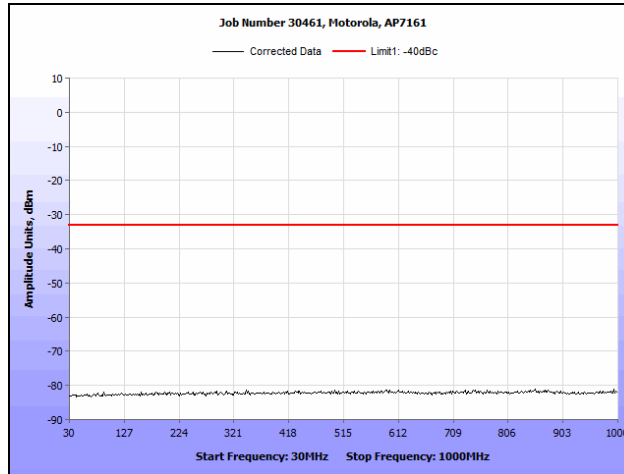
Plot 65. Conducted Spurious Emissions, 802.11a, 4950 MHz (30 MHz – 1 GHz), R3-A
