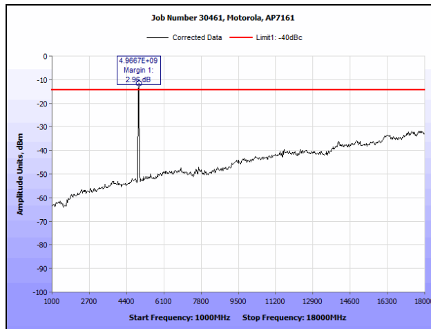
Plot 146. Radiated Spurious Emissions, 802.11a, 4960 MHz (1 GHz – 18 GHz), (1x1)
