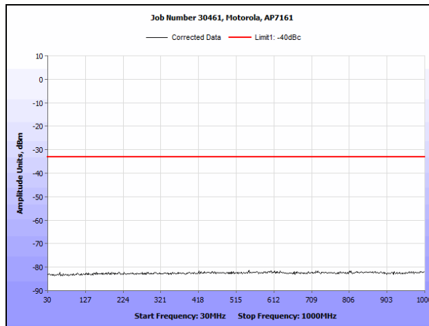
Plot 115. Conducted Spurious Emissions, 802.11n HT20, 4970 MHz (30 MHz - 1 GHz), R3-B
