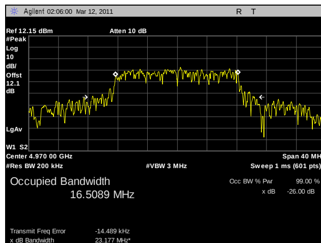
Plot 9. Emission Bandwidth, 802.11a, 4970 MHz, Port C (3x3)
