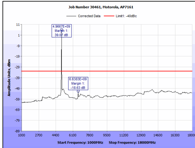
Plot 116. Conducted Spurious Emissions, 802.11n HT20, 4970 MHz (1 GHz – 18 GHz), R3-B
