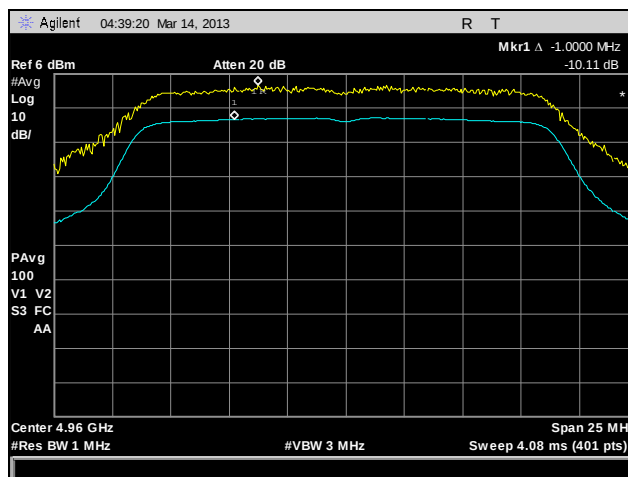
Plot 169. Peak Excursion, 802.11n HT20, 4960 MHz, Port B
