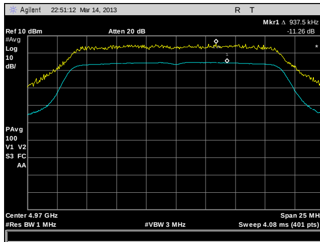
Plot 183. Peak Excursion, 802.11n HT20, 4970 MHz, 1x1
