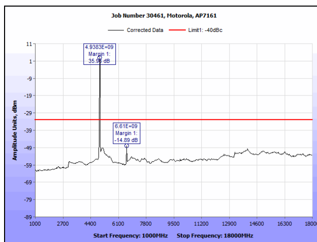
Plot 100. Conducted Spurious Emissions, 802.11n HT20, 4950 MHz (1 GHz – 18 GHz), R3-B
