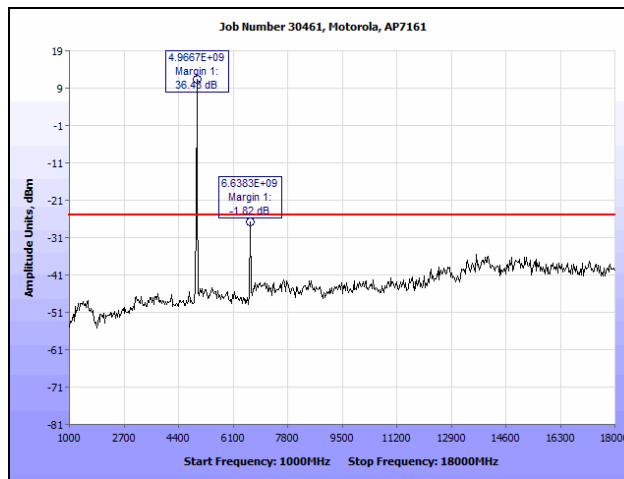
Plot 120. Conducted Spurious Emissions, 802.11n HT20, 4970 MHz (1 GHz – 18 GHz)
