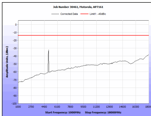
Plot 140. Radiated Spurious Emissions, 802.11n HT20, 4960 MHz (1 GHz – 18 GHz)
