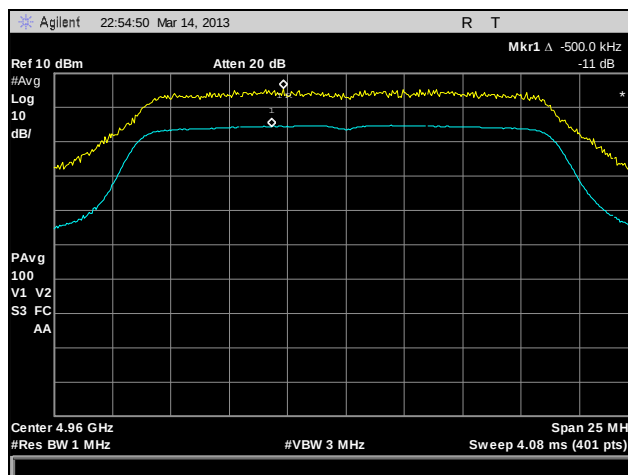
Plot 182. Peak Excursion, 802.11n HT20, 4960 MHz, 1x1
