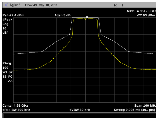
Plot 33. Emission Mask, 802.11a, 4950 MHz, Port A (3x3)
