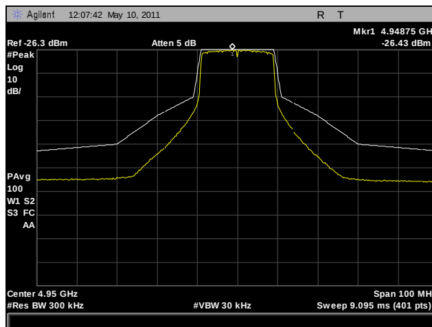
Plot 47. Emission Mask, 802.11n HT20, 4950 MHz, Port C (3x3)
