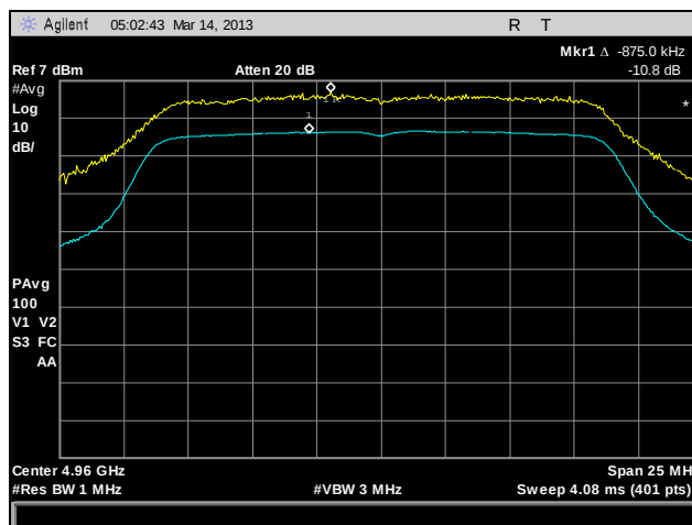
Plot 170. Peak Excursion, 802.11n HT20, 4960 MHz, Port C
