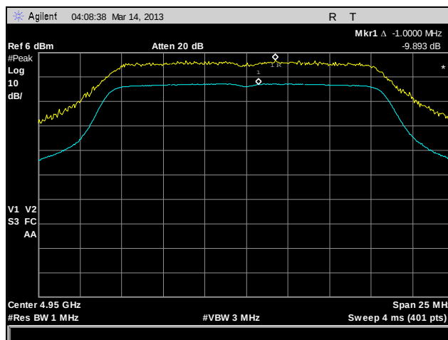
Plot 154. Peak Excursion, 802.11a, 4950 MHz, Port B
