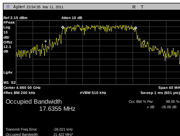
Plot 23. Emission Bandwidth, 802.11n HT20, 4980 MHz, Port B (3x3)
