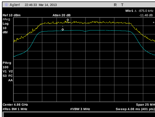
Plot 180. Peak Excursion, 802.11a, 4980 MHz, 1x1
