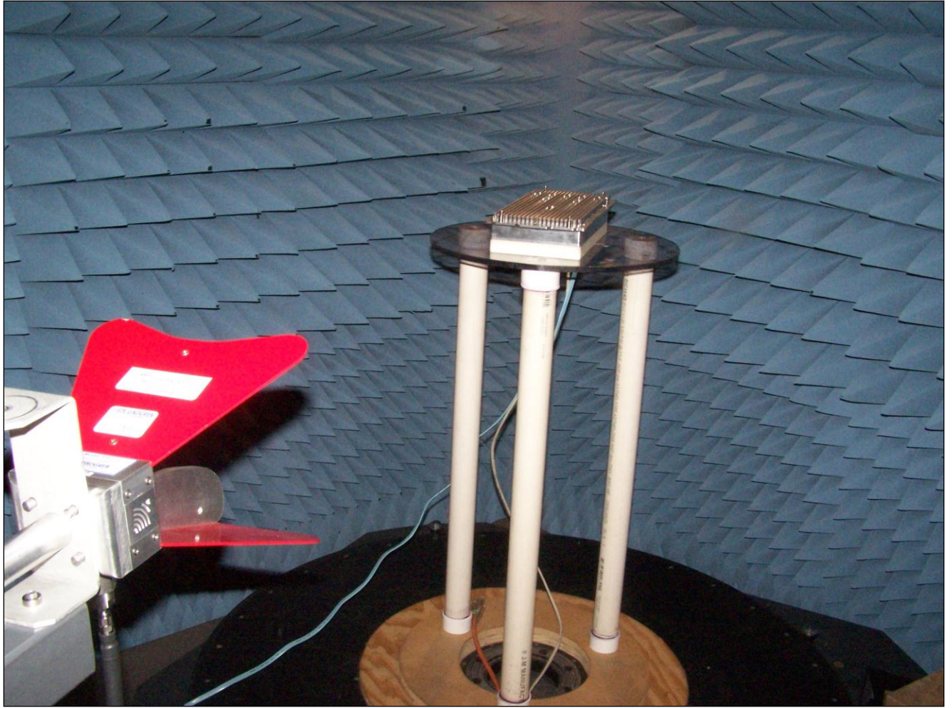
Photograph 3. Radiated Spurious Emissions, Test Setup
