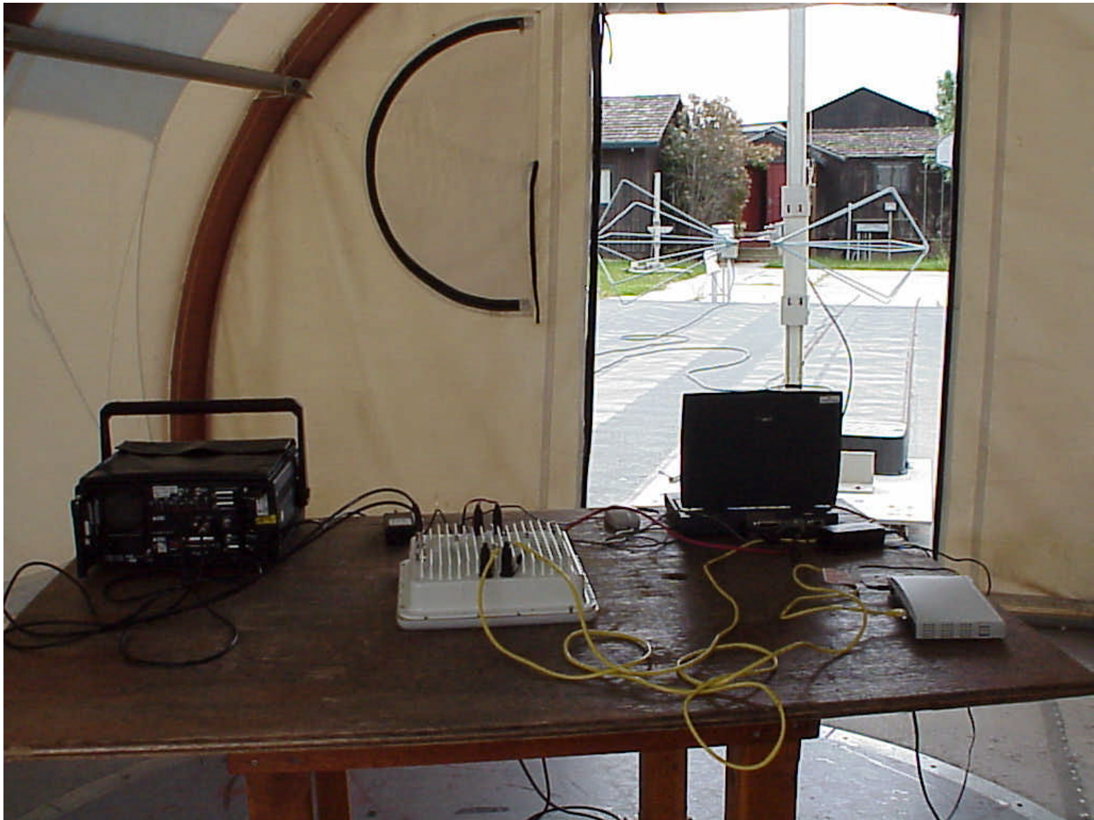
Link CX, 15.209 radiated measurement setup, 30 MHz to 1 GHz
