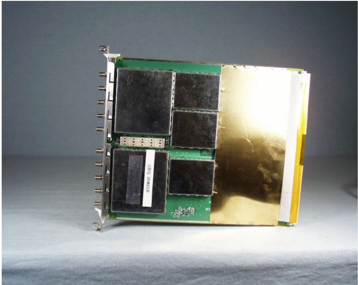
Side view of the 340119 RF Distribution Module
