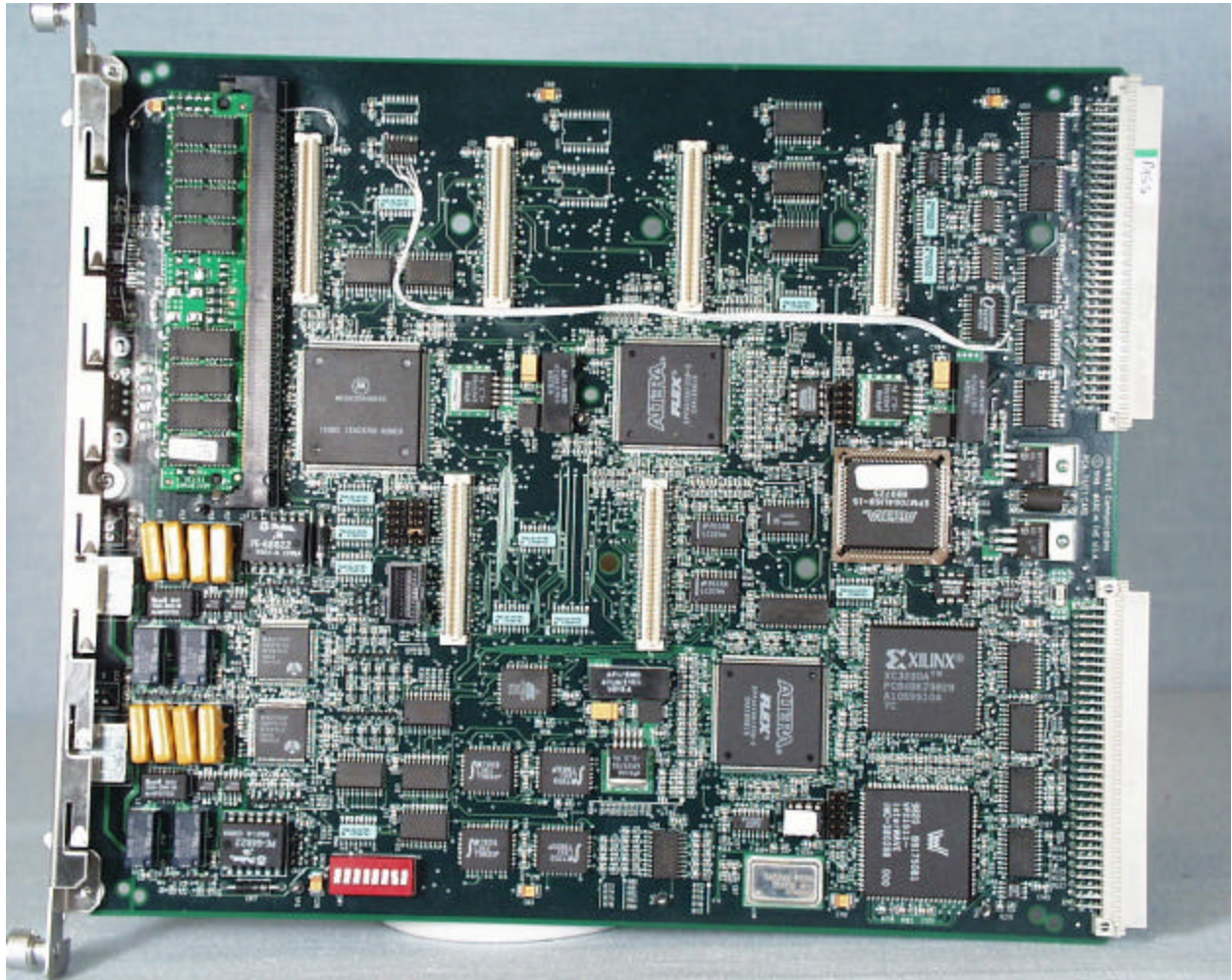
Side view of the 340122 2-port E1/T1 Interface board
