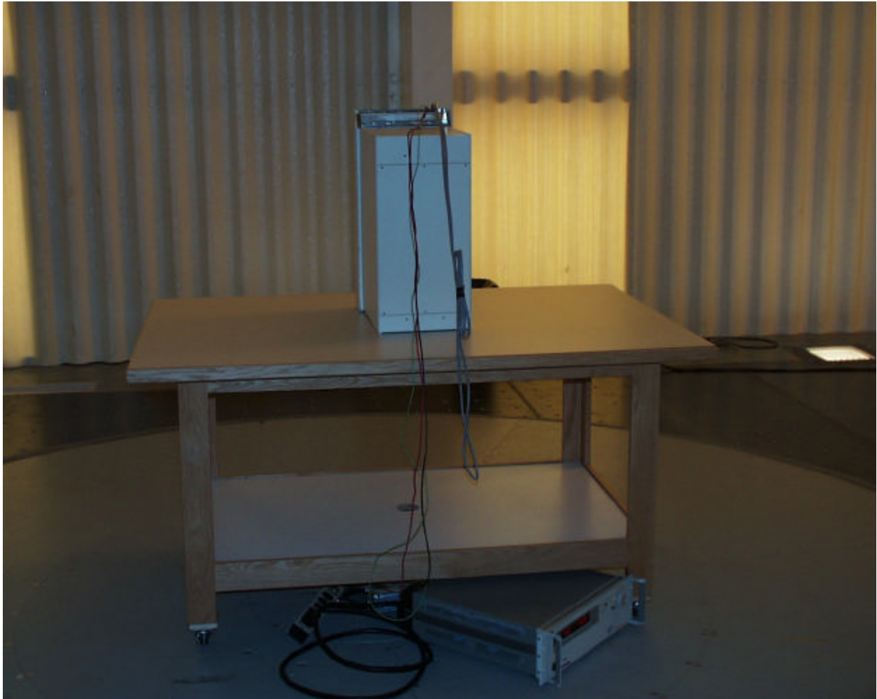
Back view of worst case radiated emissions
