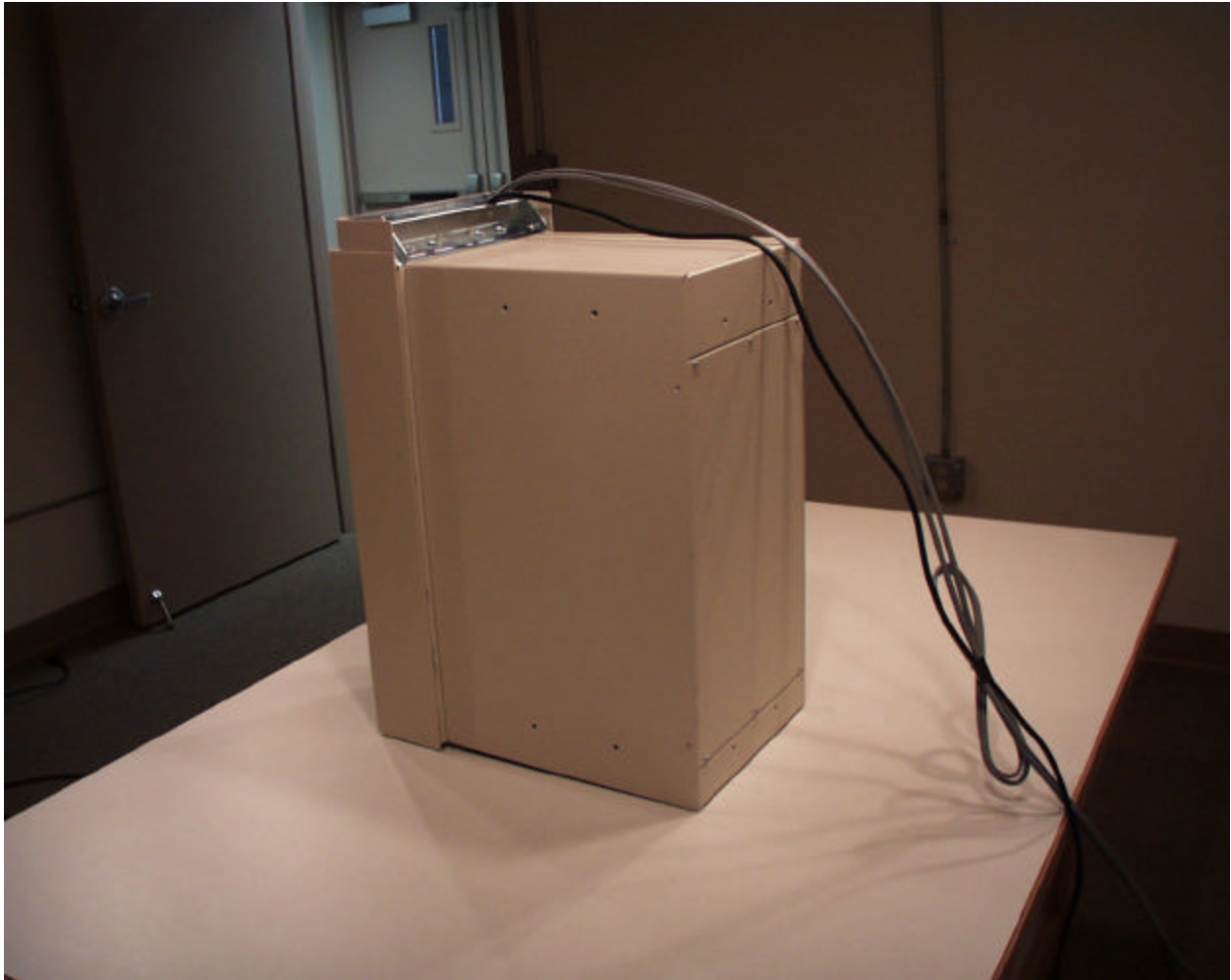
Back view of worst case line conducted emissions
