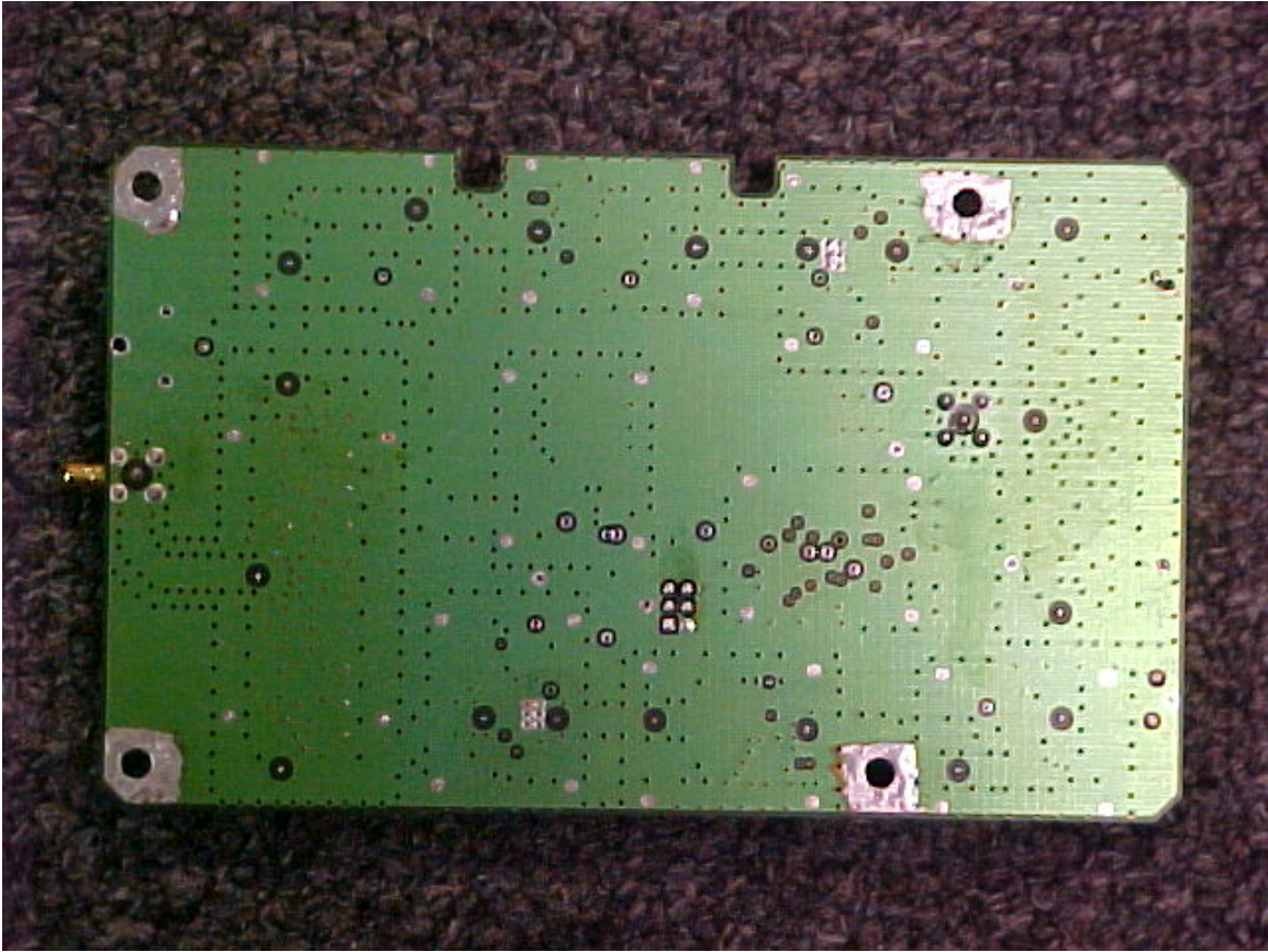
In-Home Cellular Signal Enhancer, Internal Bottom Side Circuit Board
