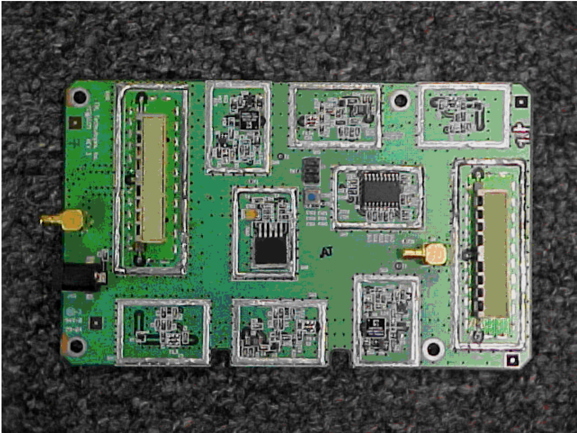
In-Home Cellular Signal Enhancer, Internal Top Side Circuit Board Shields Removed
