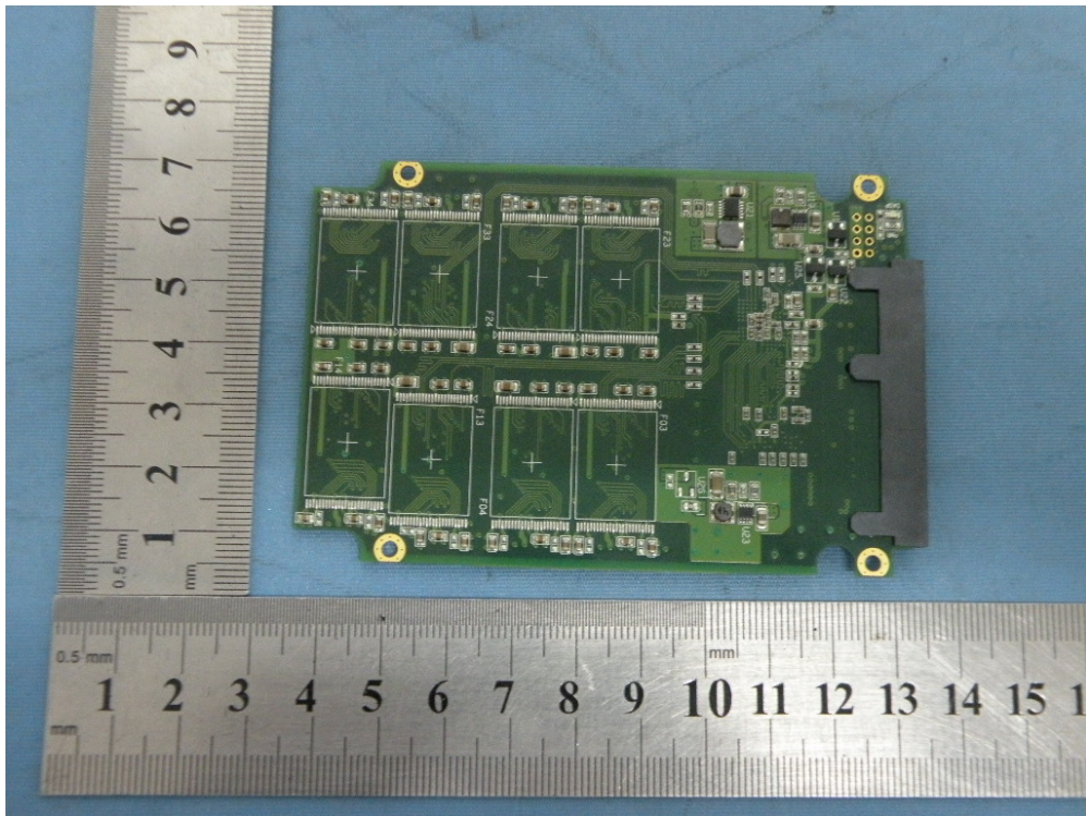
Bottom View
