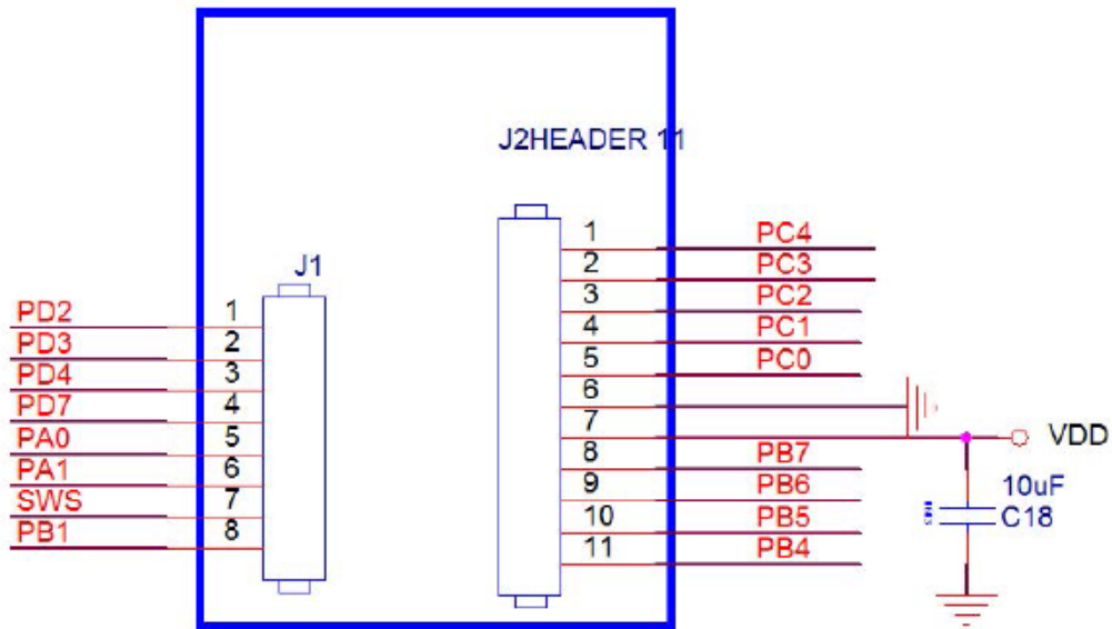
Figure 1 Pin layout
