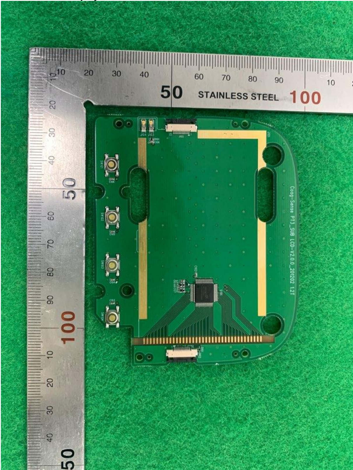
Front View of Display Board
