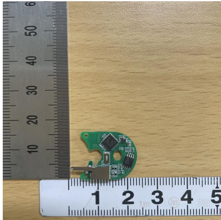
Rear View of Main Board
