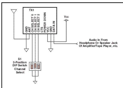
Figure 20: Typical Application: Voice Transmitter
