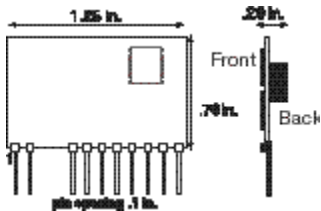
Figure 10: Physical package
