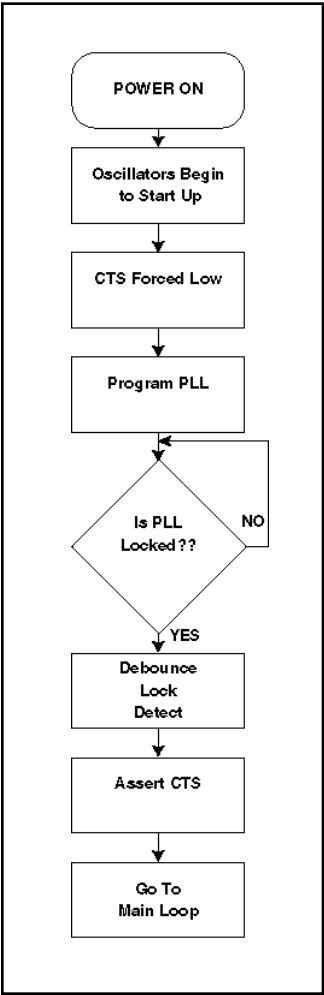
Figure 16: Start-up sequence
