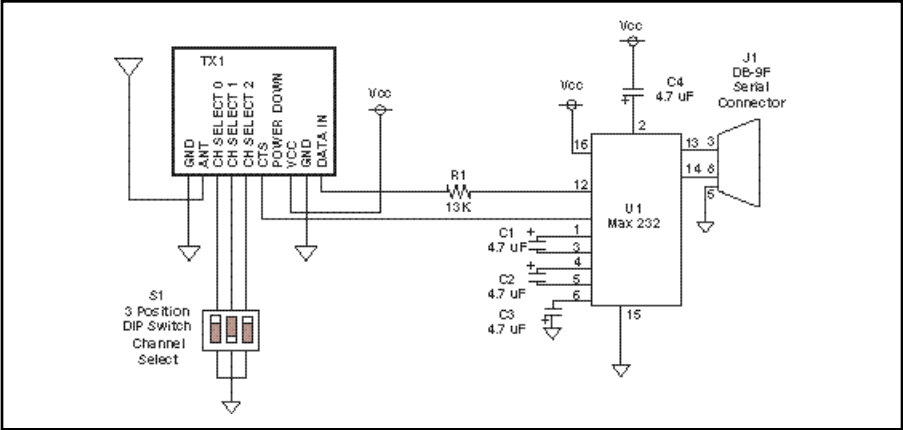
Figure 18: Typical Application: RS-232 Interface
