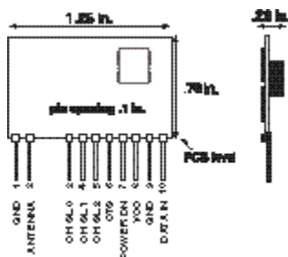
Figure 1: Physical Dimensions
