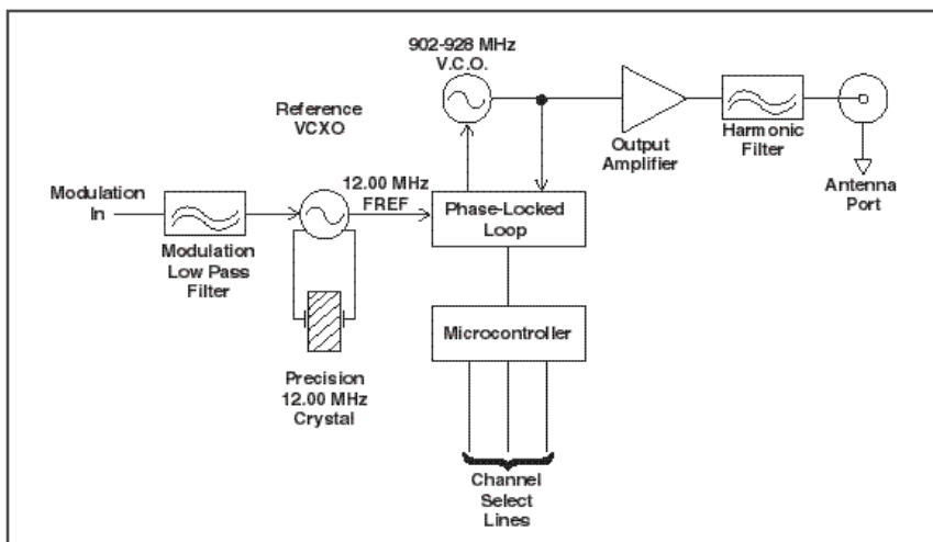
Figure 12: HP Series transmitter block diagram
