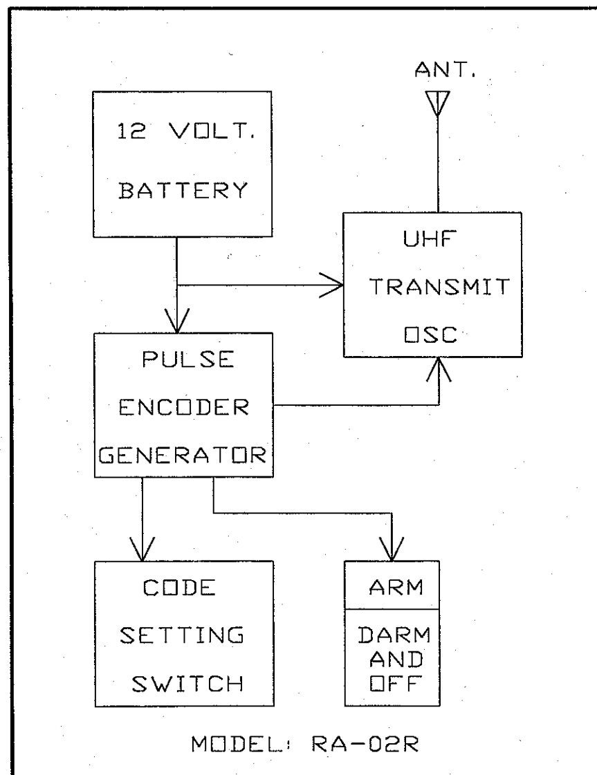
2-KEYS REMOTE CONTROL TRANSMITTER
