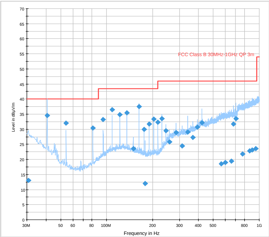
Radiated spurious emissions 30 MHz to 1 GHz
