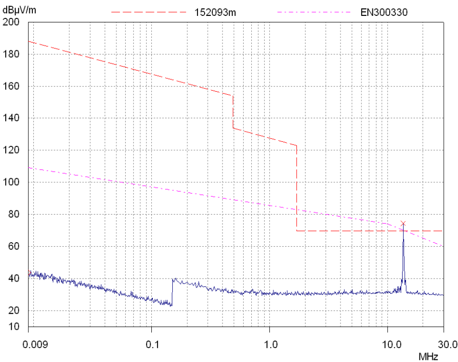
Radiated spurious emissions 9kHz to 30MHz
