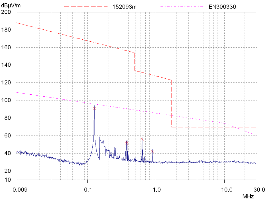
Radiated spurious emissions 9 kHz to 30 MHz
