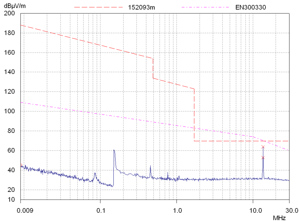
Radiated spurious emissions 9 kHz to 30 MHz
