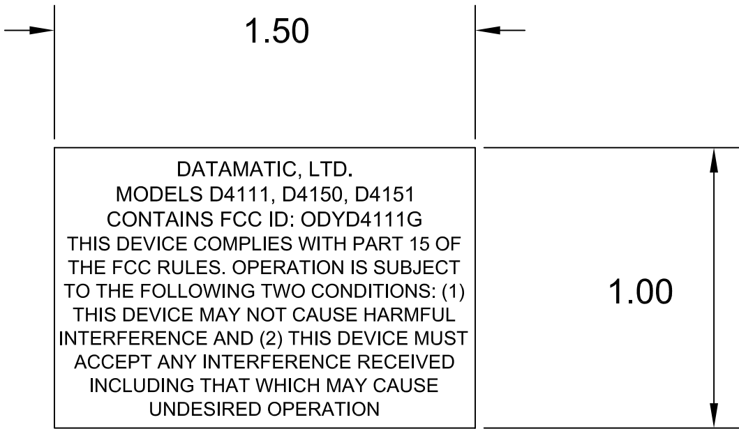
INCH DIMENSIONS
