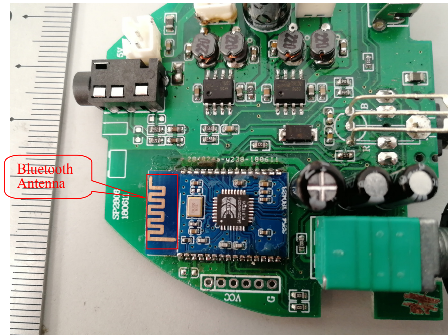
EUT – PCB Antenna View
