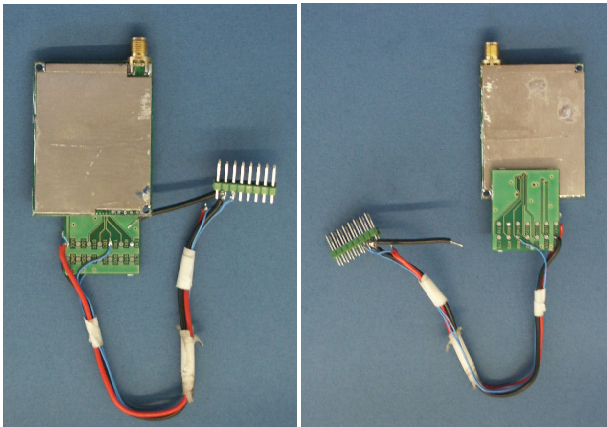
Fig. 10: Front and back view of the device with cable for the power supply and PC connection.
