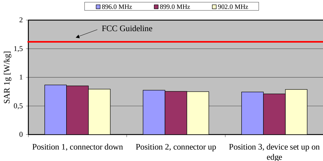
Fig. 7: The measured SAR values in body-worn configuration for the Advantra AR100 in the 900 MHz range in comparison to the FCC exposure limit.
