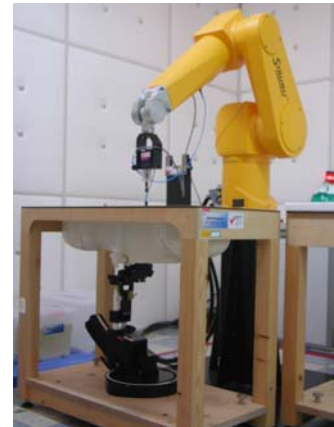
Figure 1. SAR System
