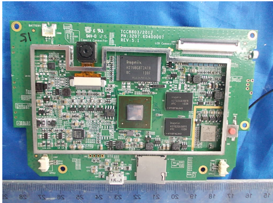
FIGURE 2 VINCI LEARNING TABLET (M/N: VINCI TAB) MAIN BOARD (COMPONENT SIDE)
