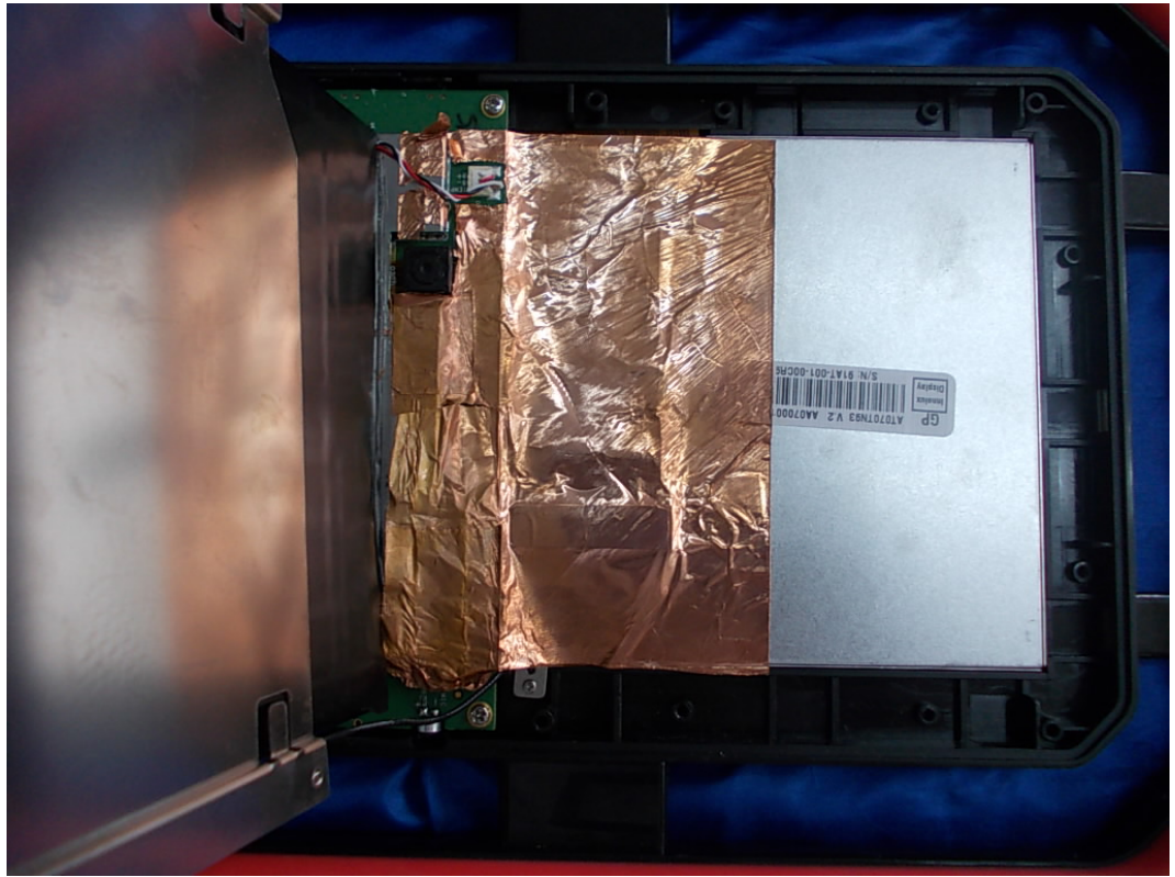
FIGURE 8 VINCI LEARNING TABLET (M/N: VINCI TAB) DEBUG
