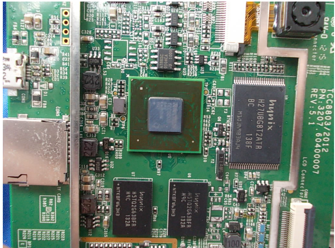
FIGURE 4 VINCI LEARNING TABLET (M/N: VINCI TAB) CPU
