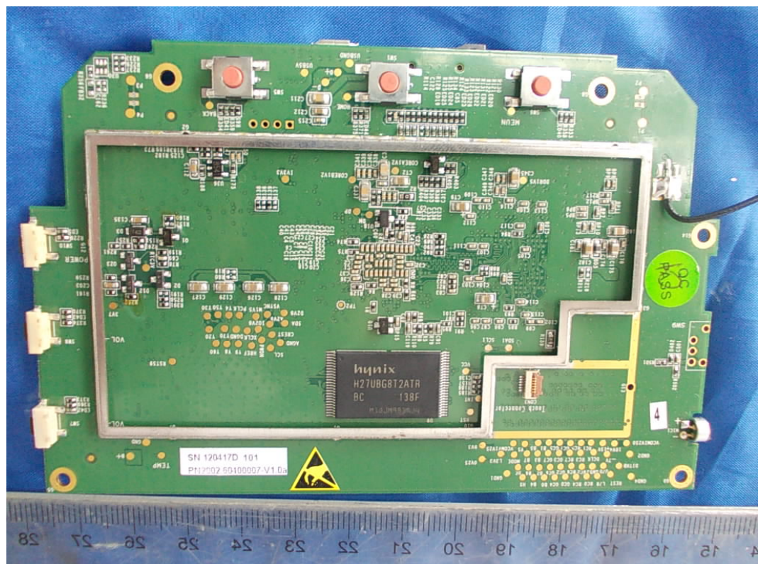
FIGURE 3 VINCI LEARNING TABLET (M/N: VINCI TAB) MAIN BOARD (SOLDERED SIDE)
