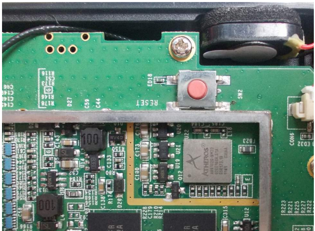
FIGURE 7 VINCI LEARNING TABLET (M/N: VINCI TAB) RF PART ON MAIN BOARD
