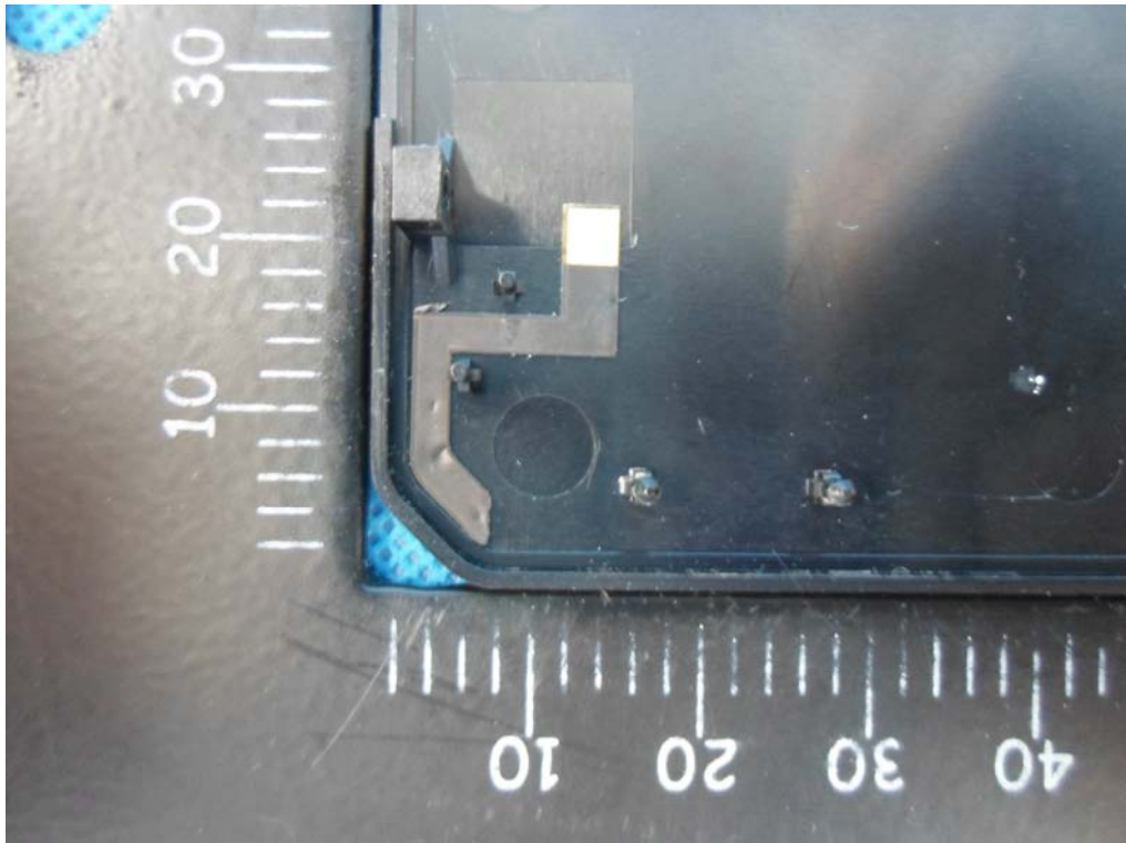
Photo 17 WiFi Antenna
