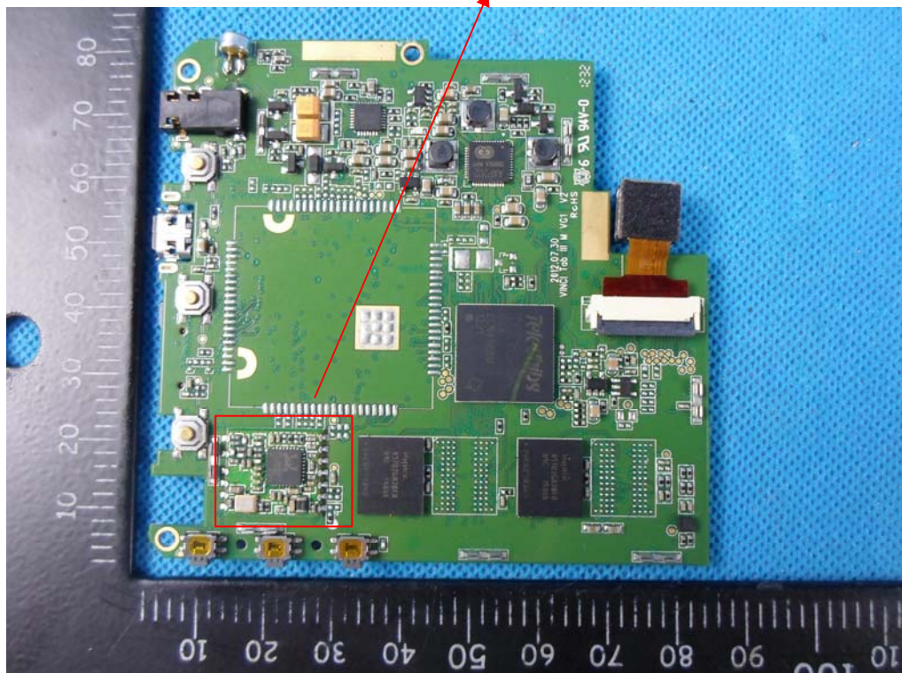
Photo 14 WiFi Module
