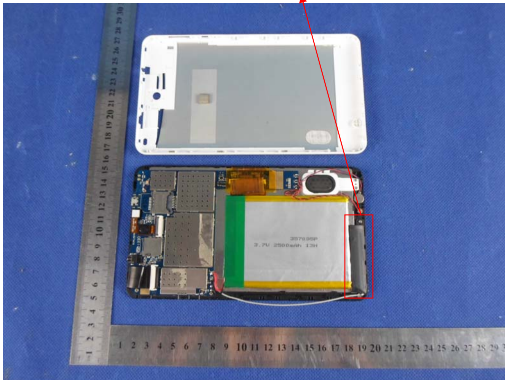
Photo 8 Wwan Antenna.
