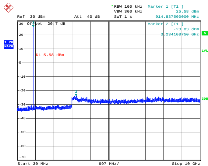
Figure 7.4.2.2-4: 30 MHz – 10 GHz – Low Channel - Antenna port 1
