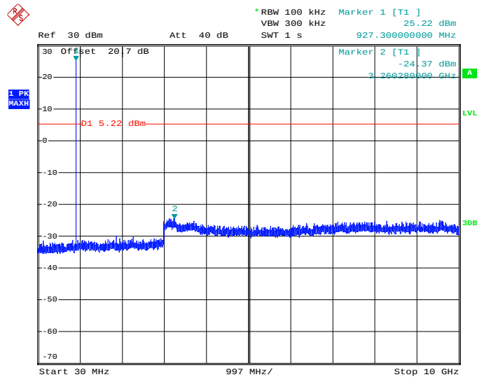
Figure 7.4.2.2-2: 30 MHz – 10 GHz – Middle Channel - Antenna port 0
