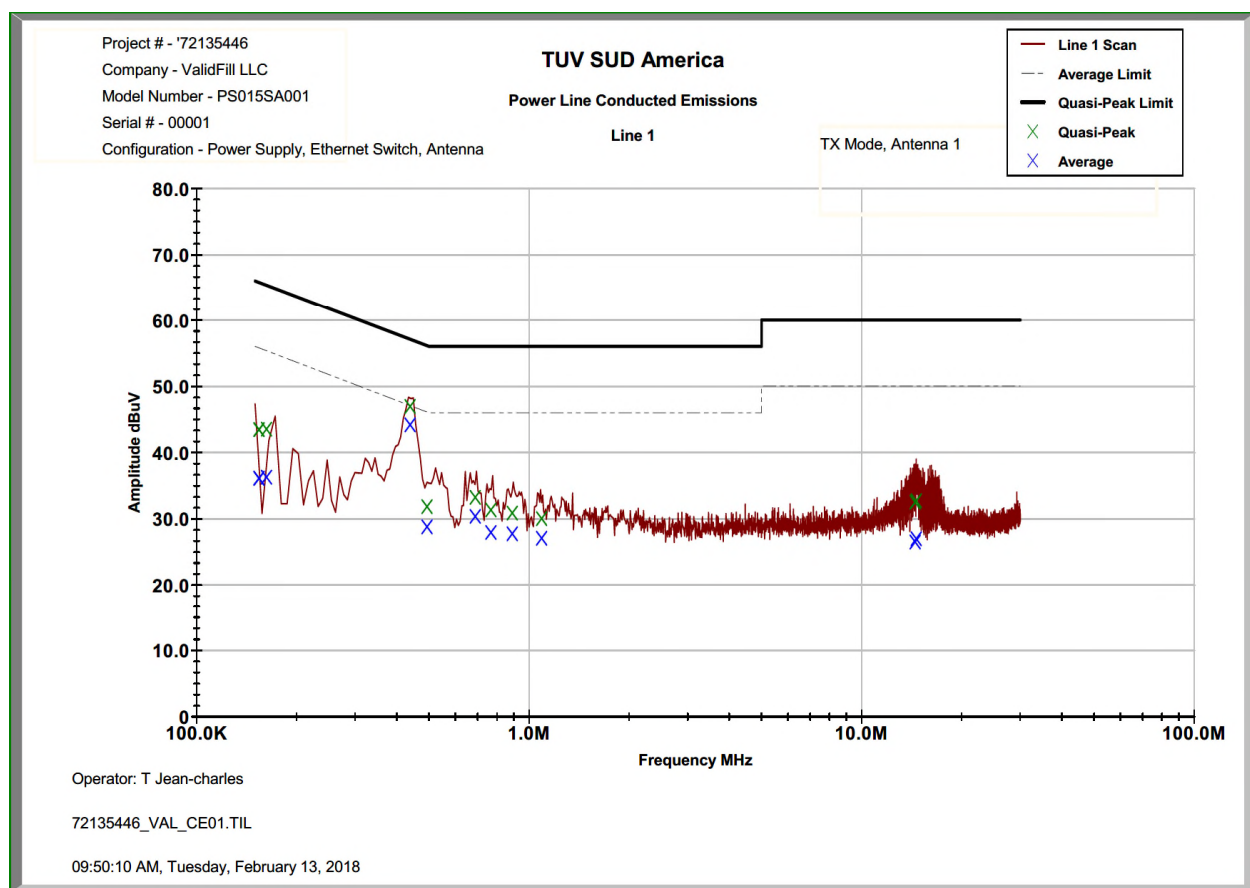
Figure 7.5.2-1: Conducted Emissions Results – Line 1
