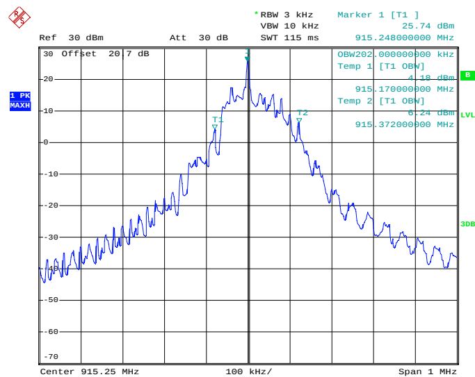
Figure 7.3.4.2-4: 99% BW – Low Channel - Antenna port 0
