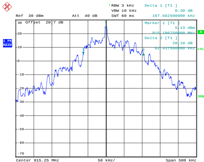
Figure 7.3.4.2-7: 20 dB BW – Low Channel - Antenna port 1
