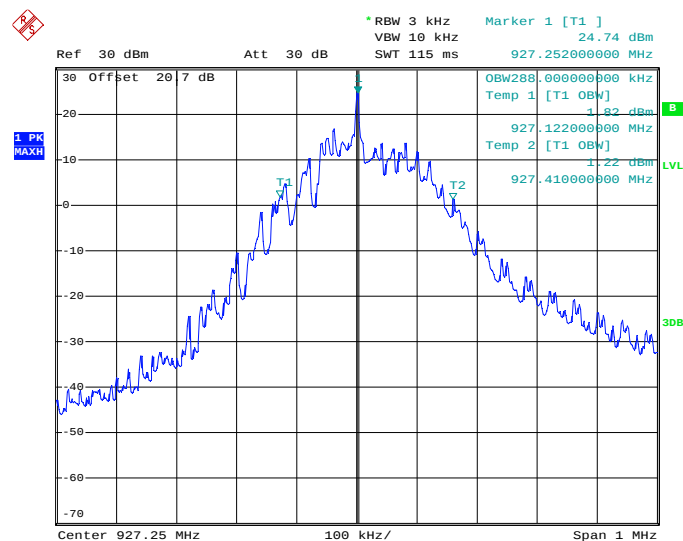
Figure 7.3.4.2-11: 99% BW – Middle Channel - Antenna port 1
