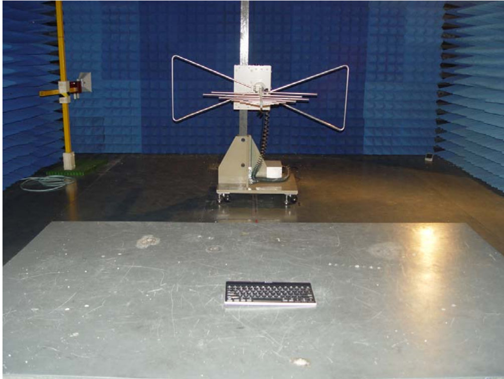
Radiated emissions test 30MHz- 1GHz
