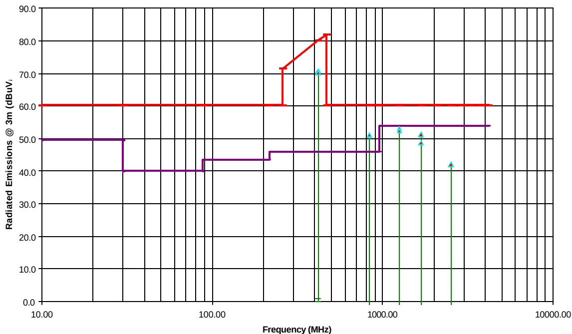
Radiated Emissions Measurements @ 3m OFTS CANSEC ACCESS CONTROL TRANSMITTER, MODEL SF-100
