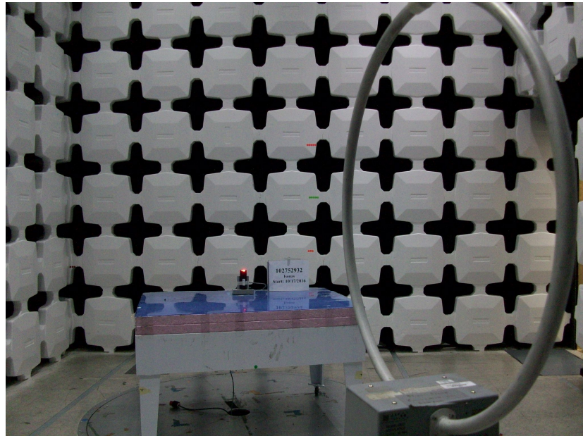
Test Setup – Front (9kHz – 30MHz)
