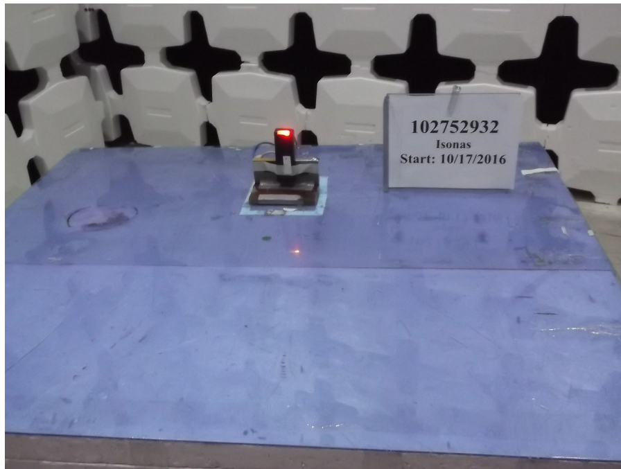
Test Setup – Axis 1
