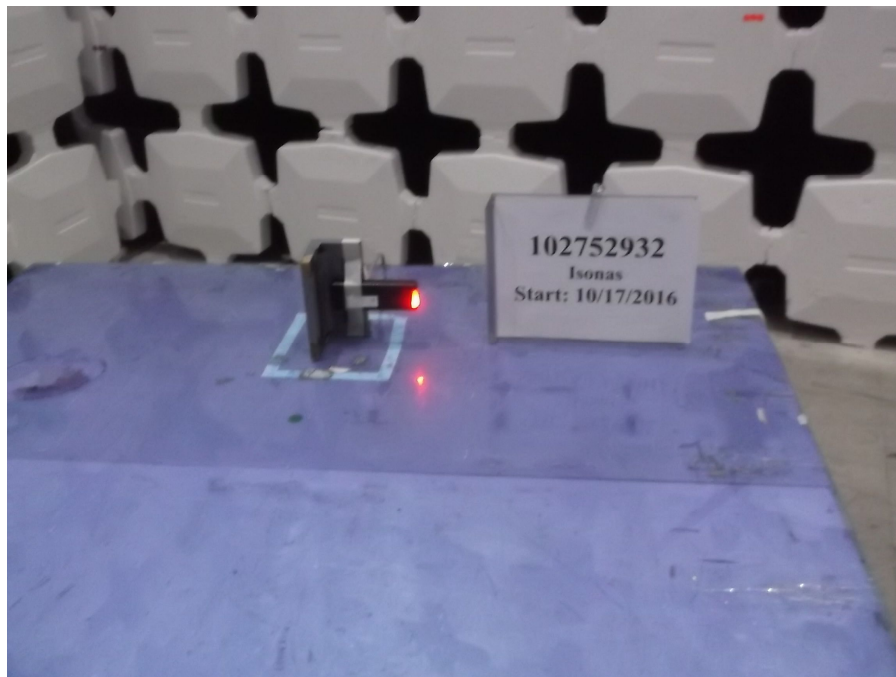
Test Setup – Axis 2
