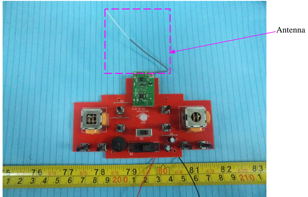
EUT – Main Board & RF Module Board Top View
