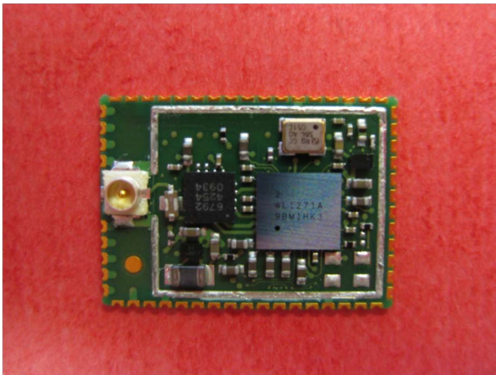
RF Module (Without Shield)
