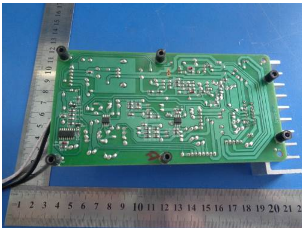
PCB Board 3– Rear View
