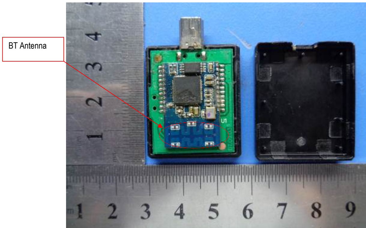
Cover Off - Top View 1
