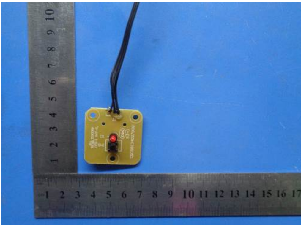
EUT PCB Board 9 - Front View
