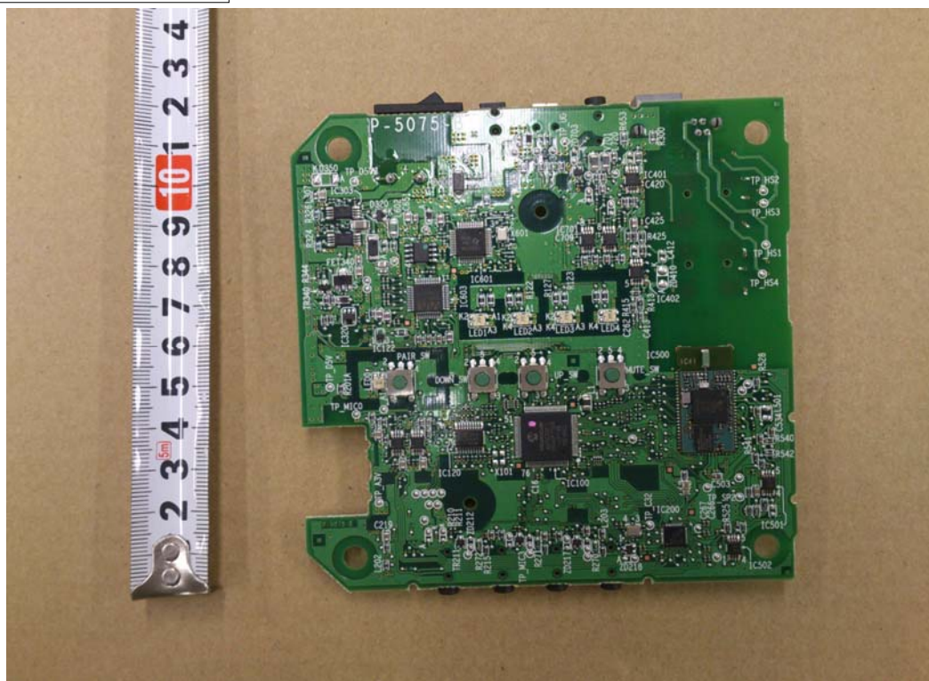
R-Talk 800EX Solder surface
