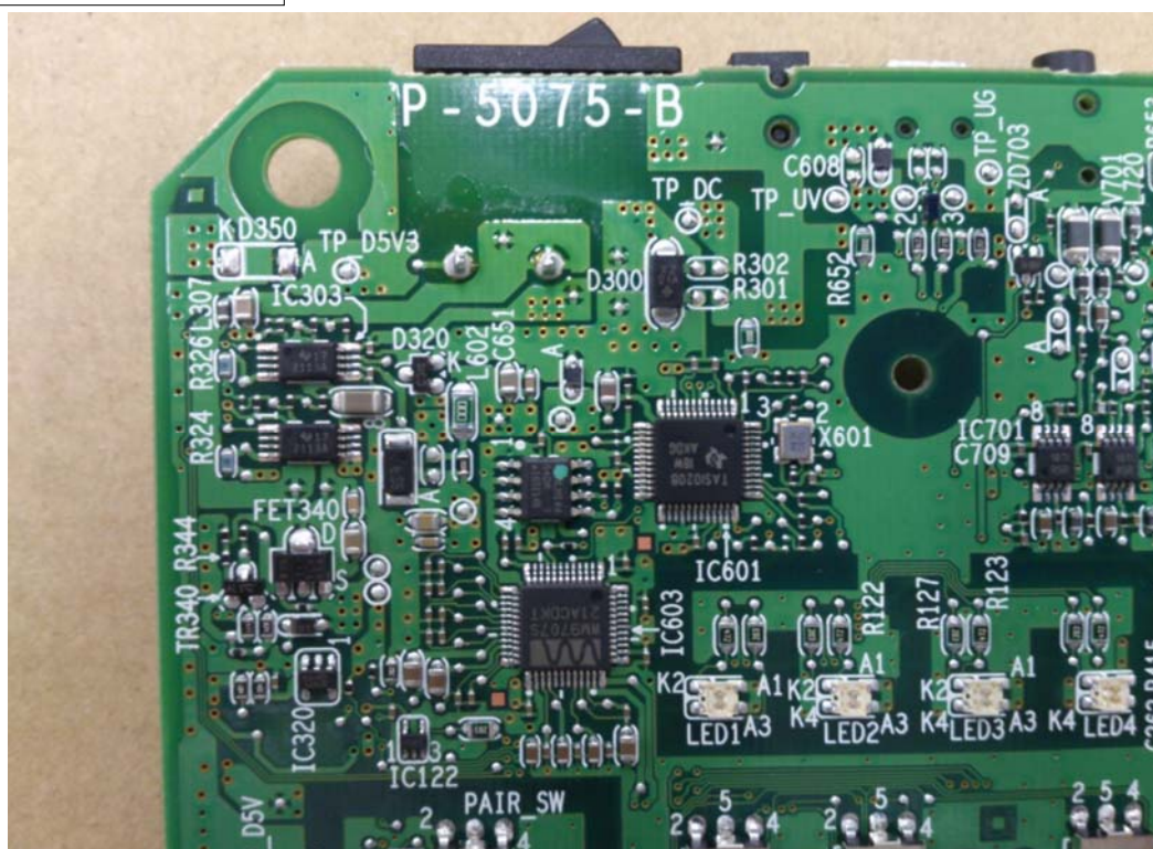
R-Talk 800EX Solder surface (Lower left)
