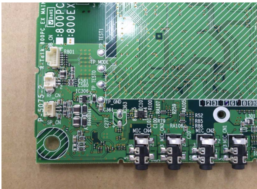
R-Talk 800EX Mounting surface (Lower left)
