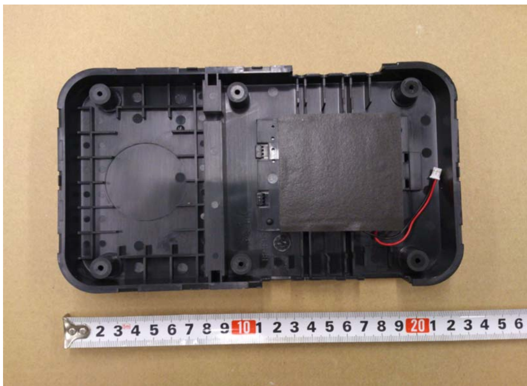
R-Talk 800EX Inside the product(Lower case)
