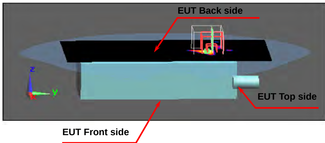
Figure 7. Body SAR Test Setup (Flat Section)
