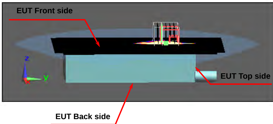
Figure 6. Body SAR Test Setup (Flat Section)
