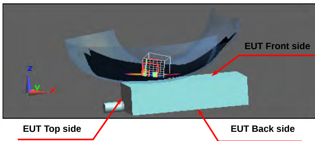
Figure 2. Right Head SAR Test Setup (Cheek)
