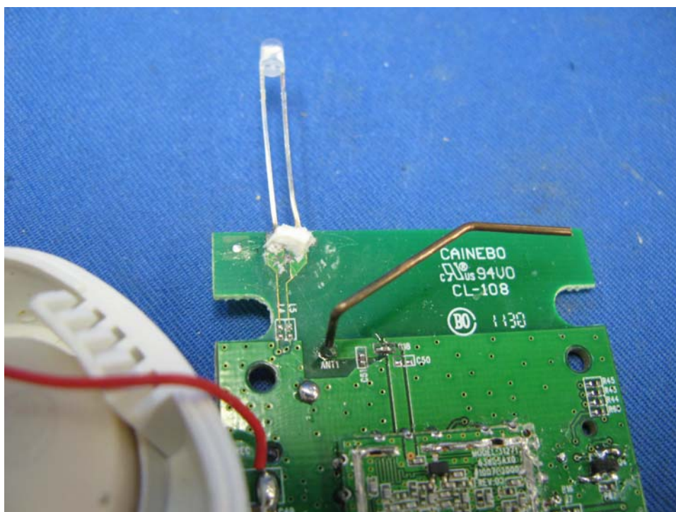
Handset Antenna
