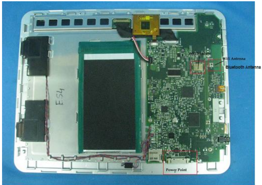
Position of the antenna with RF Module
