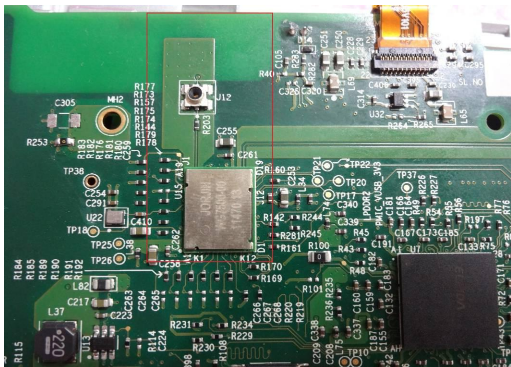
Position of the antenna with RF Module form the Bottom View as marked in Square
