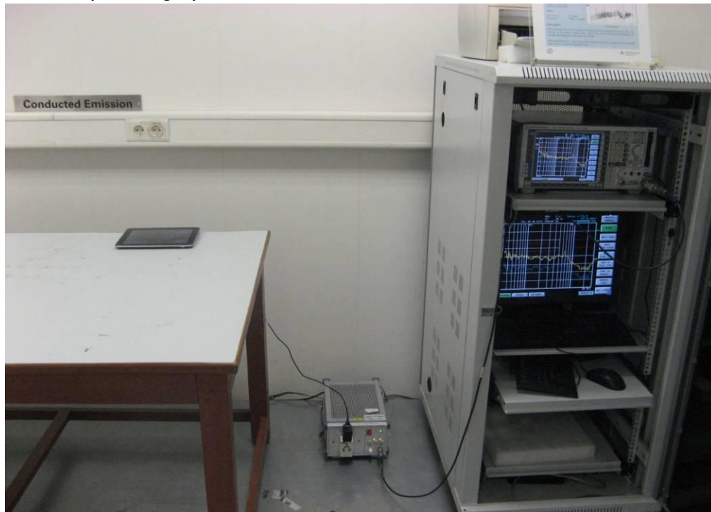
Test setup Photograph - Conducted Mains Emissions setup
