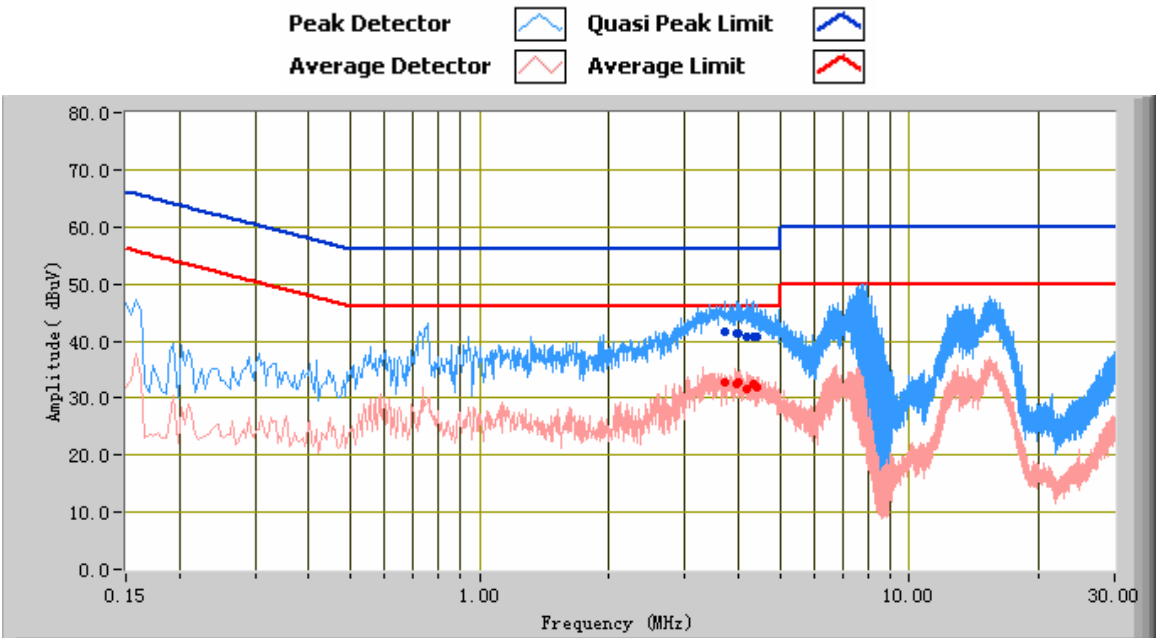
Test Data Phase Neutral Plot at 120Vac, 60Hz
