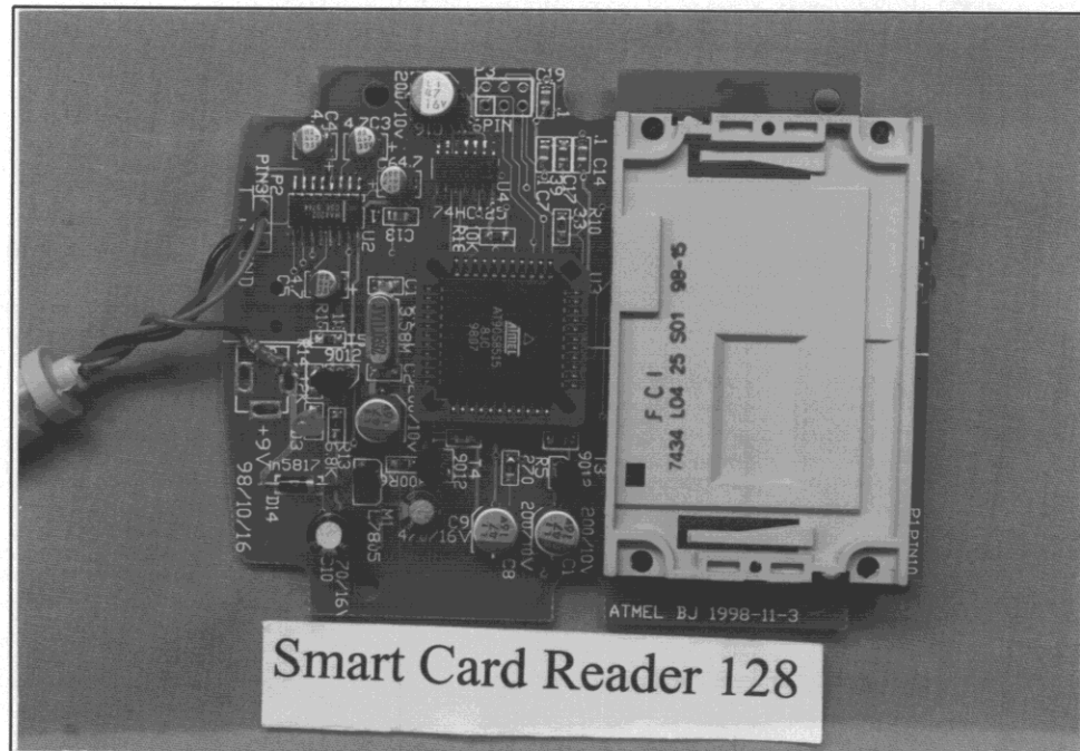
FIGURE 4 MAIN BOARD (COMPONENT SIDE)
