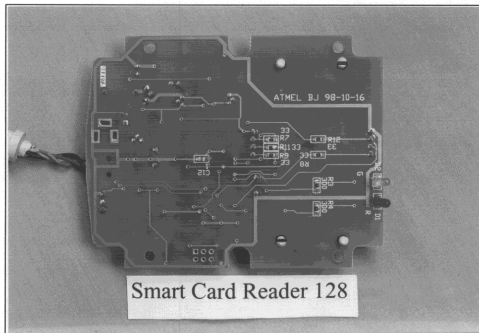
FIGURE 5 MAIN BOARD (SOLDERED SIDE)
