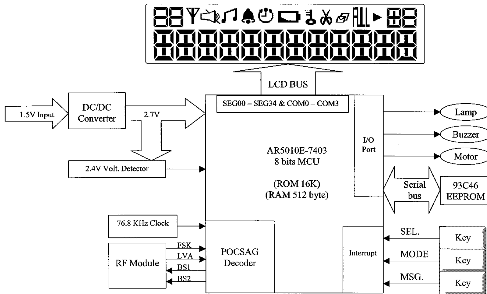
Figure 1 Block diagram of 8022N digital module
