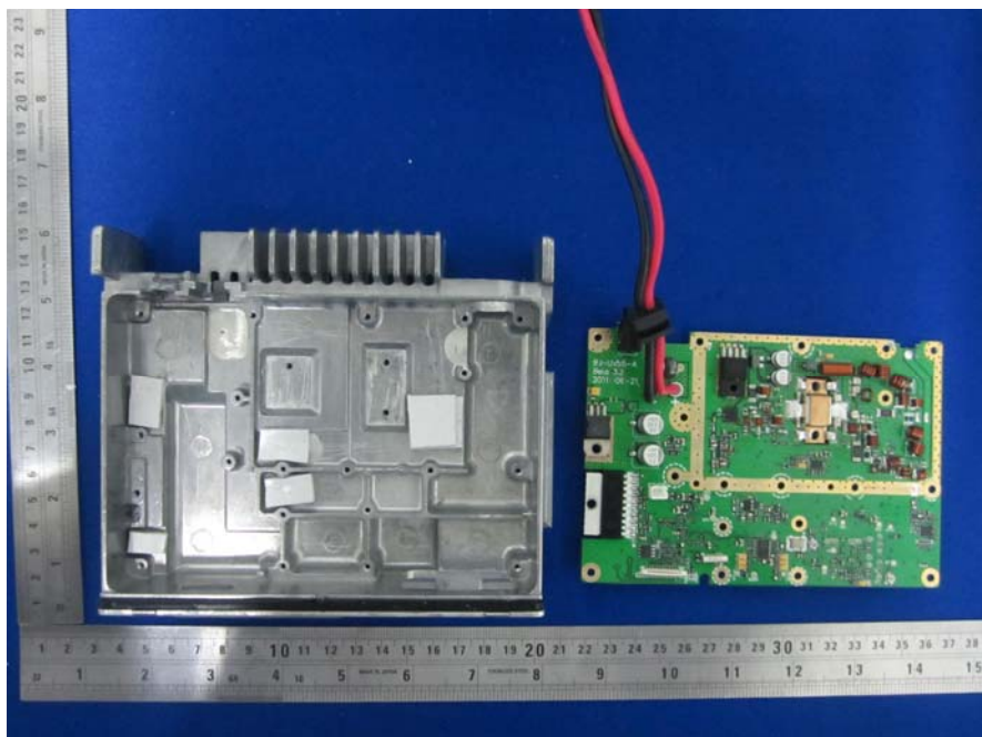
EUT –LCD Cover off View
