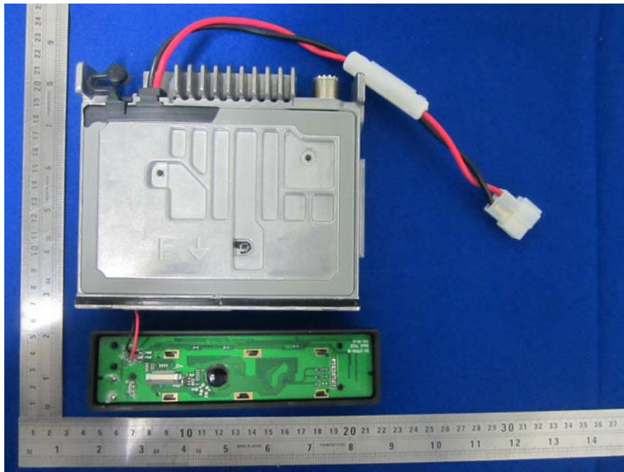
EUT –Top Shell Cover off View
