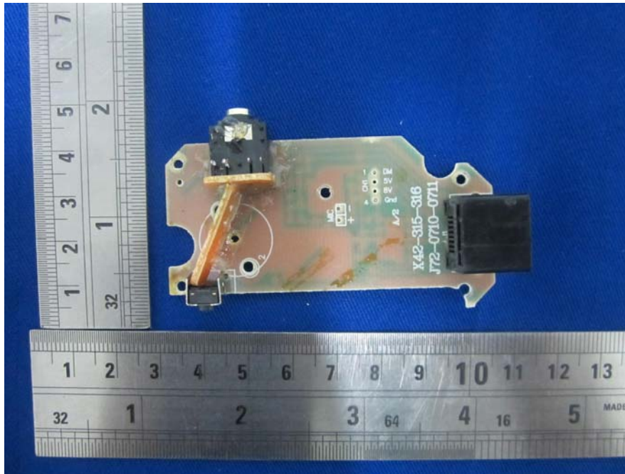
EUT –MIC Phone Board Bottom View
