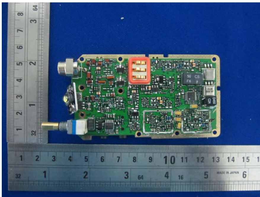
EUT – PCB Board Top Without Cover View
