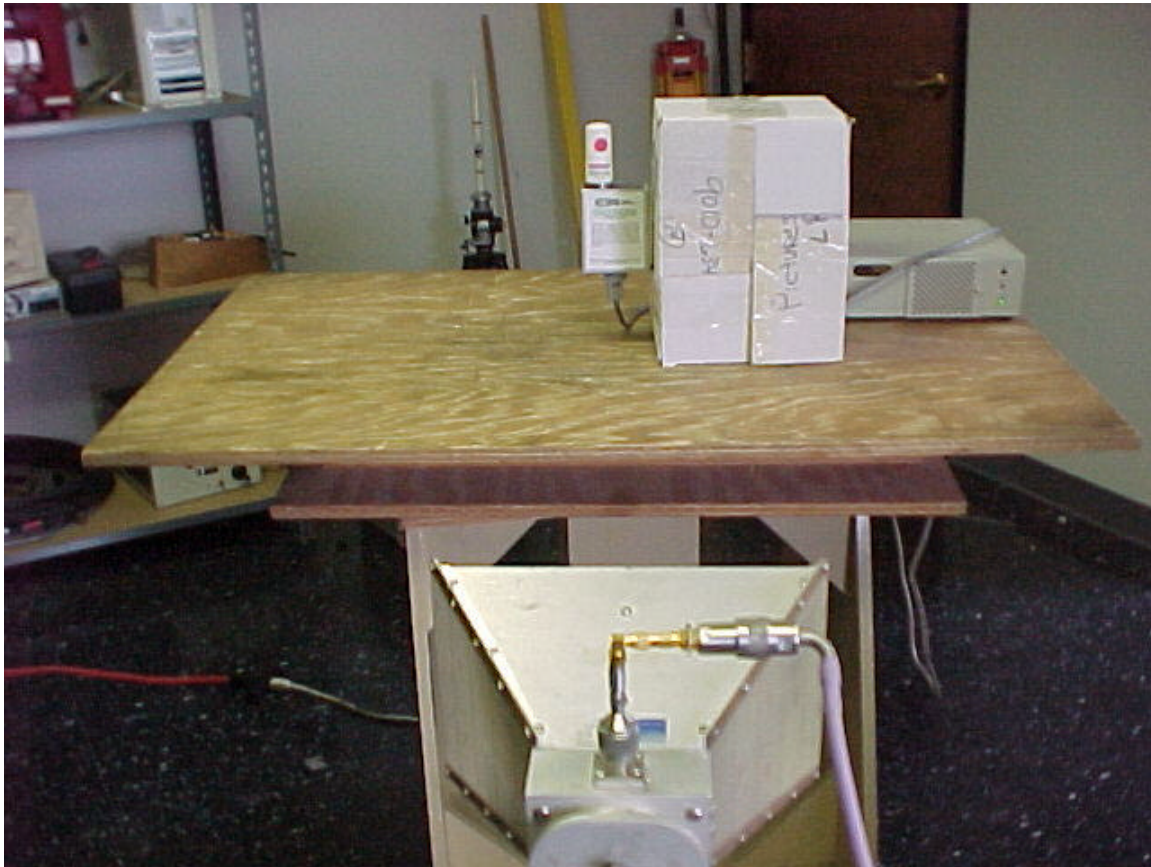
RADIATED EMISSIONS, HIGH FREQ. – FRONT OF UNIT
