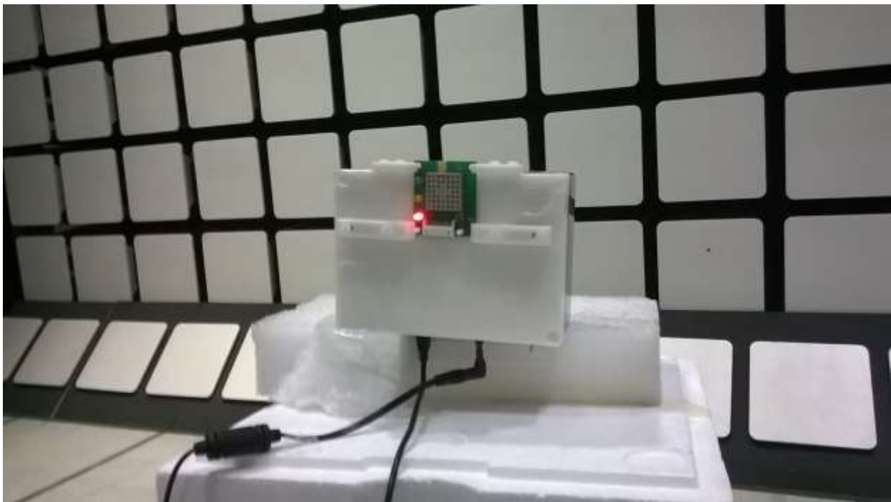
Figure 4 - Radiated emissions test setup, 1GHz - 25GHz
