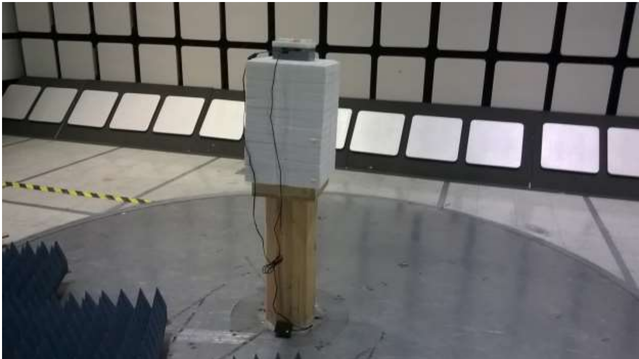
Figure 2 - Radiated emissions test setup, 1GHz - 25GHz
