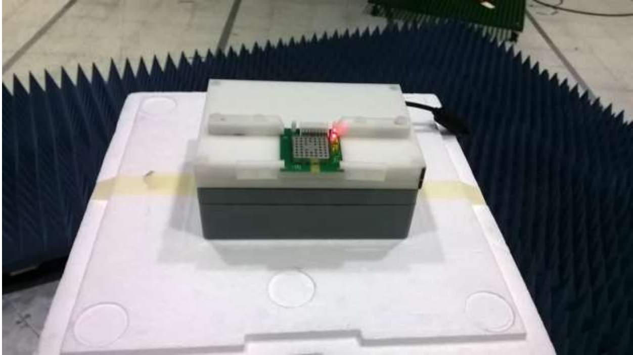
Figure 1 - Radiated emissions test setup, 1GHz - 25GHz
