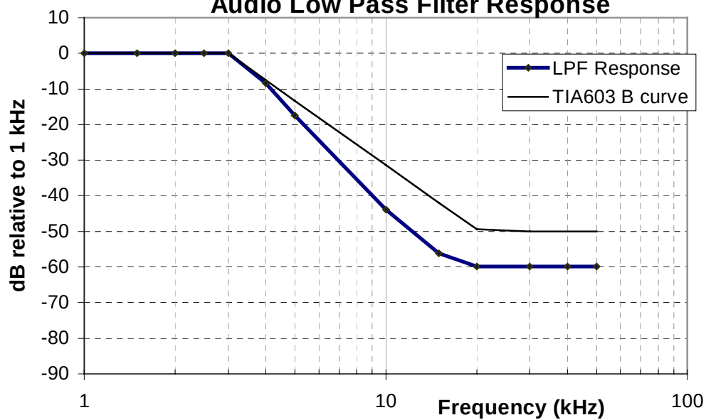
Audio Low Pass Filter Response
